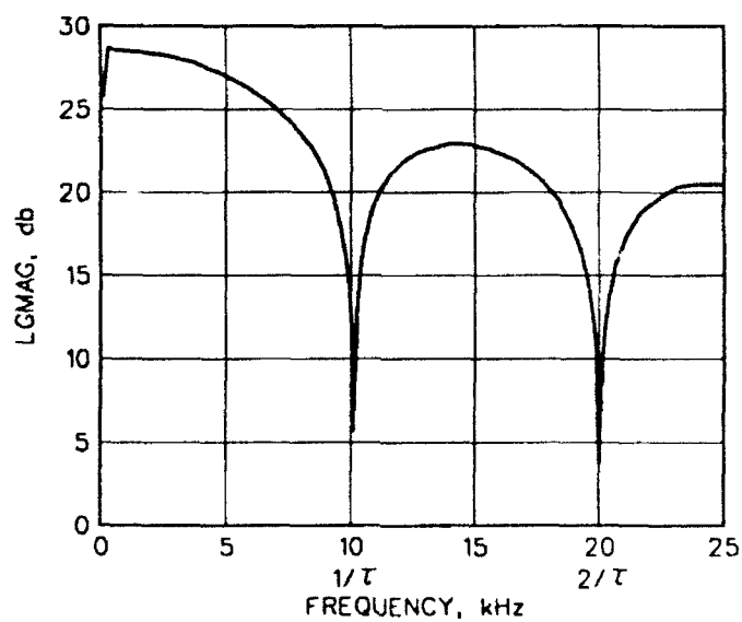
Figure 21. Frequency spectrum of rectangular pulse from a pulse generator
