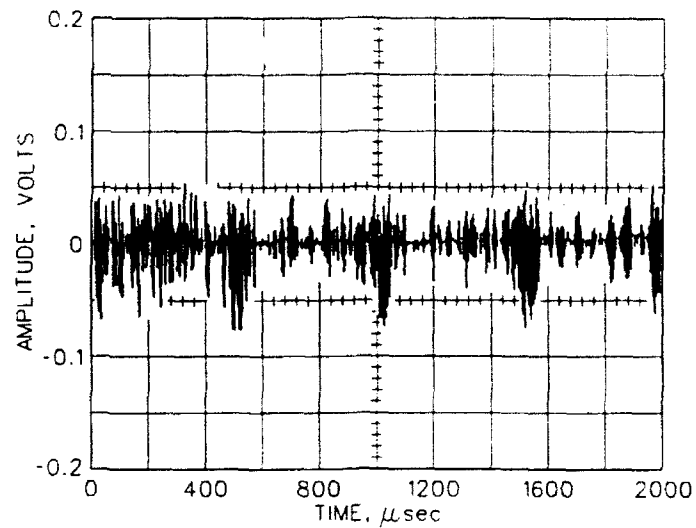
Figure 57. Ultrasonic pulse-echoes on 3-ft beam yields equally spaced echoes of approximately 500 \mu sec. Frequency of energy is 750 kHz
