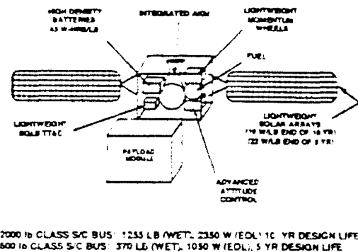
Figure 6. Generic Common Bus Configuration
