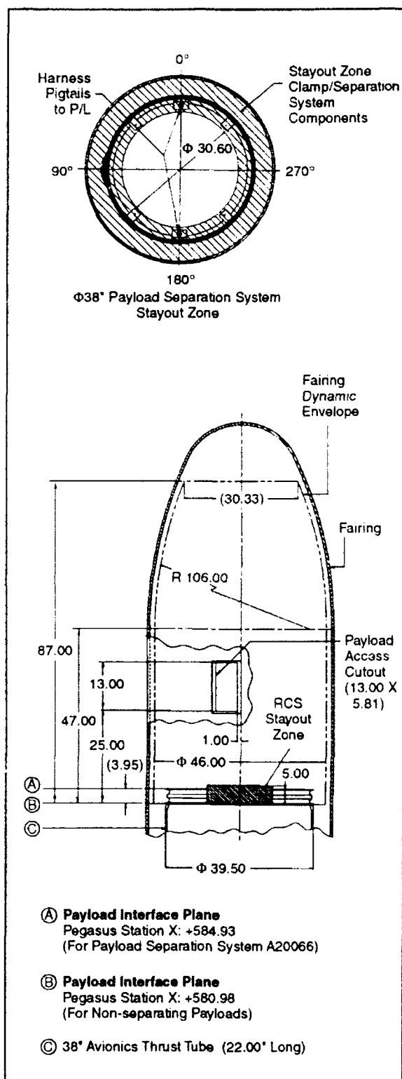
Figure 6. Standard and XL payload fairing dynamic envelope with 38" diameter payload interface.
