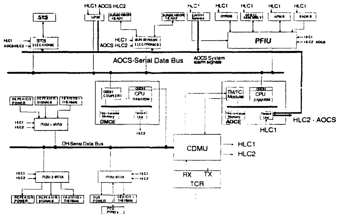
Fig. 4.3-1: ICDS principle block diagram for separated AOCS and payload DM
