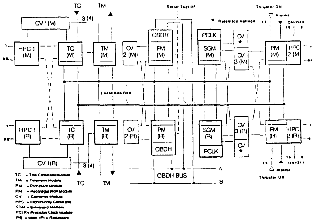
Fig. 4.3-2: Block diagram of the OBCU
