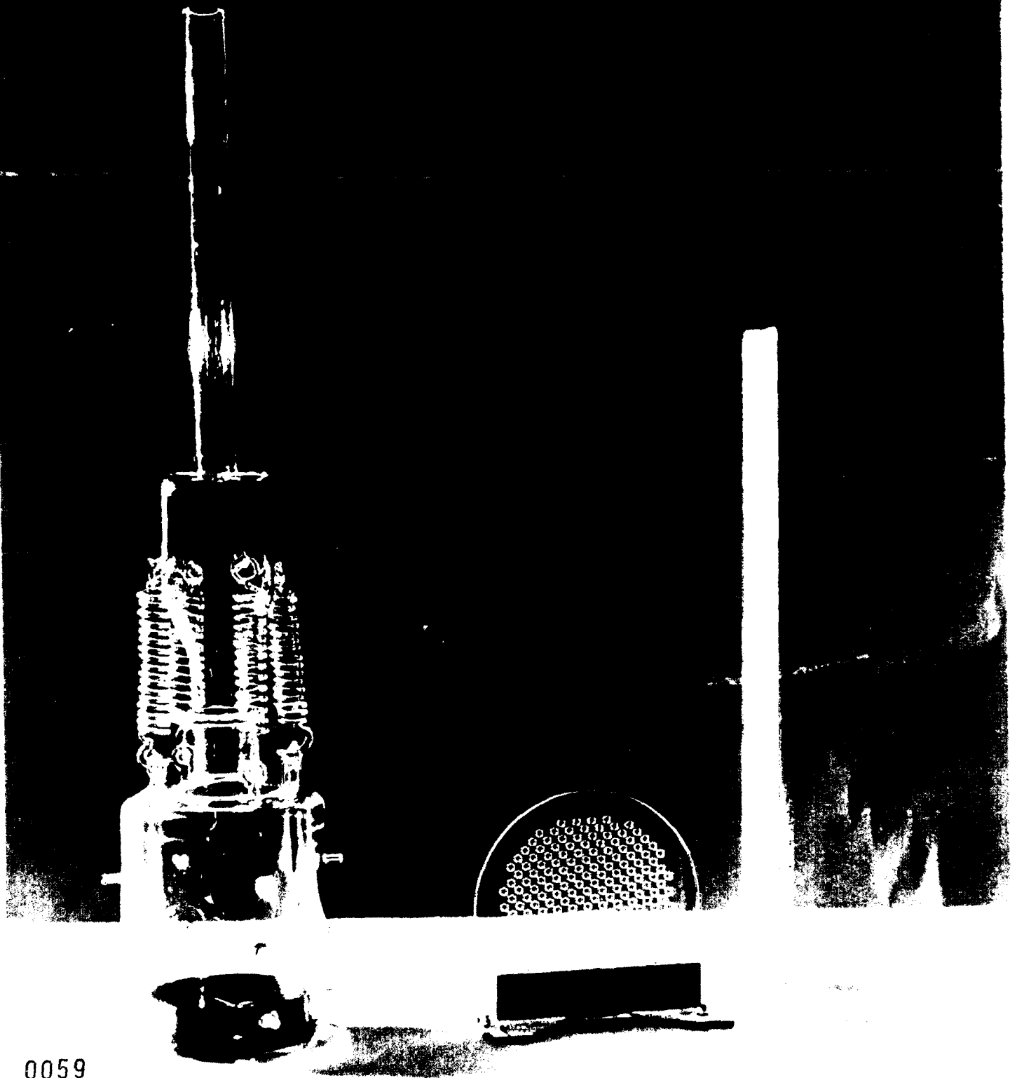
Fig. 6. Quartz Vaporization and Ionization Chamber Held Together by Tension Springs
