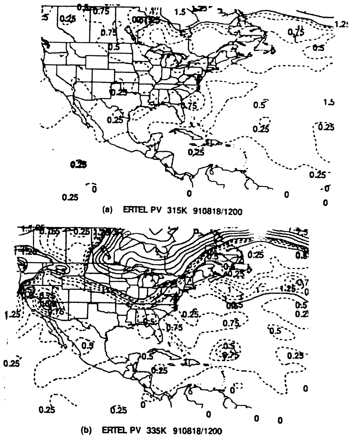
Fig. A-1 Ertel potential vorticity (PV) at 12 UTC 18 August 1991 on the (a) 315°K and (b) 335°K isentropic surface (Wu and Emanuel 1993). Potential vorticity values smaller than (larger than or equal to) 1.5 PVU are shown as dashed (solid) lines with unequal contour intervals of 0.25 PVU (1.5 PVU).
