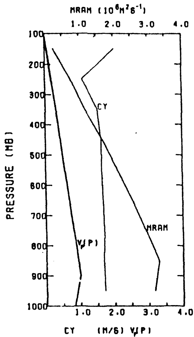
Fig. A-2 Initial tangential wind V_p (normalized by maximum wind) and mean relative angular momentum (MRAH) variations with pressure in the Wang and Li (1992) 10-level numerical model. Mean meridional drift speed C_y of the vortex at 24 h is also shown.
