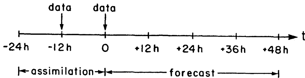
Fig. 13 Time diagram illustrating the data assimilation procedures with initial conditions at t = -24 h, additional analyses at t = -12 h and t = 0 h. Observed boundary conditions are available from t = -24 h to t = 0 h and forecast boundary conditions from a global model are supplied from t = 0 h to t = 48 h (Bennett et al. 1992).
