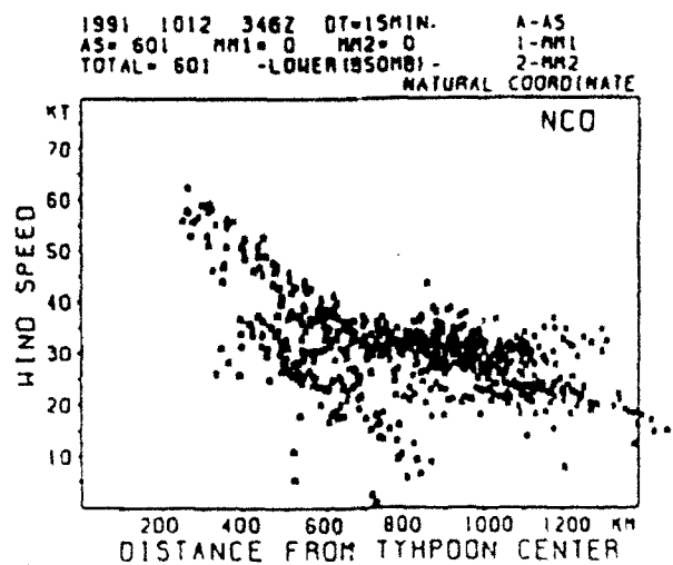
Fig. 8 (Left) Detailed low-level cloud-drift winds estimated from 15 minute GMS imagery of Typhoon Orchid (9121) at 0346 UTC 12 October 1991. (Right) Tangential wind speeds (kt) as a function of distance from the typhoon center extracted from the imagery on the left (Ohnishi 1992b).
