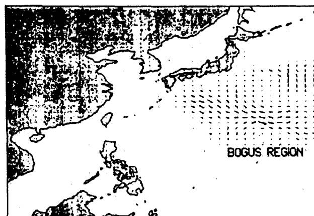
Fig. 5 (a) Original 500 mb NOGAPS wind analysis for Typhoon Zola indicating analyzed (open symbol) and actual (closed symbol) positions; (b) revised analysis following insertion of bogus vortex; and (c) analysis differences subtracting (b) from (a). Maximum vector length is 25 m s -1 (Holland et al. (1991)).
