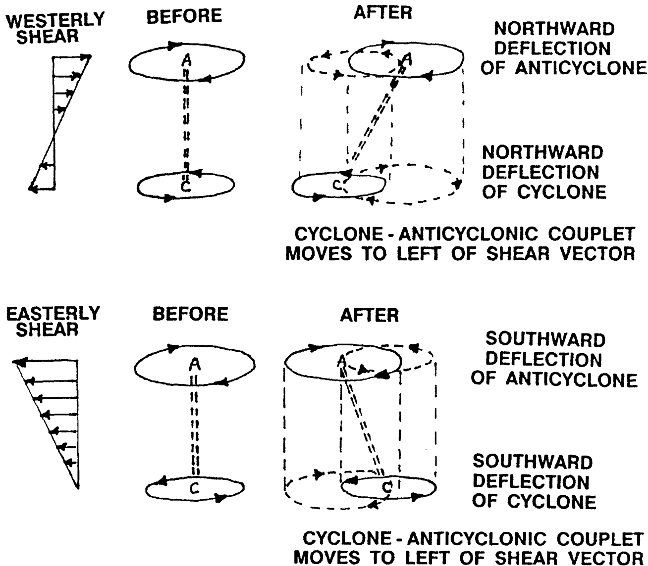
Fig. A-12 Schematic of the potential interaction between an upper-level anticyclone (A) and low-level cyclone that were initially vertically oriented (middle section), but were then exposed to a westerly shear (top) or an easterly shear (bottom). Following Wu and Emanuel (1993), the potential vorticity distributions in each layer induce circulations in the adjacent layer (dashed) lines that deflect the upper-level and lower-level circulations as indicated in the right column.
