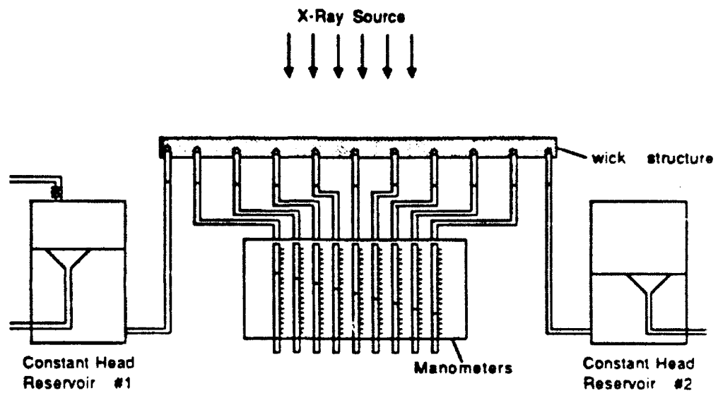
Schematic of Relative Permeability Test
