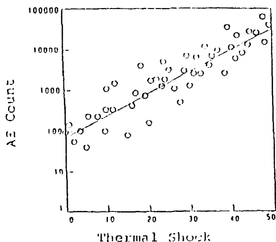
Fig. 7 AE count change monitored in a 200-layers sample of PNTT with aging time. The accelerated aging was performed by a thermal shock treatment
