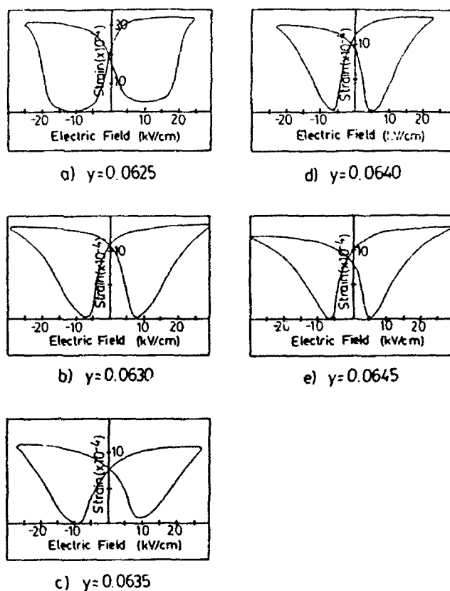
Fig. 3. Strain-vs-field characteristics in the single-plate-type samples of PNZST for various Ti mole fractions.
