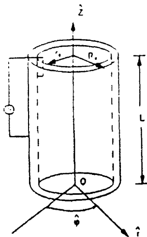
Figure 1: Schematic drawing of a radially poled ceramic tube with the outer radius R_0 and inner radius r_0 .
