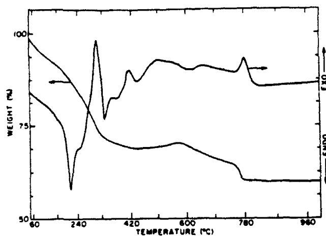
FIG. 4. TGA and DTA curves for the gel powder obtained from lanthanum acetylacetonate and titanium isopropoxide precursors (heating rate 10 °C/min).
