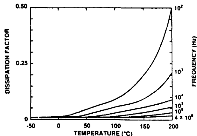
Fig. 2. Variation of the dissipation factor with temperature and frequency of the disk barrier layer capacitor of composition BP.
