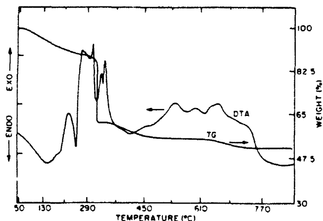
Fig. 2. TG and DTA curves for \text{SrNb}_2\text{O}_7 gel (heating rate 10^\circ\text{C}/\text{min} ).
