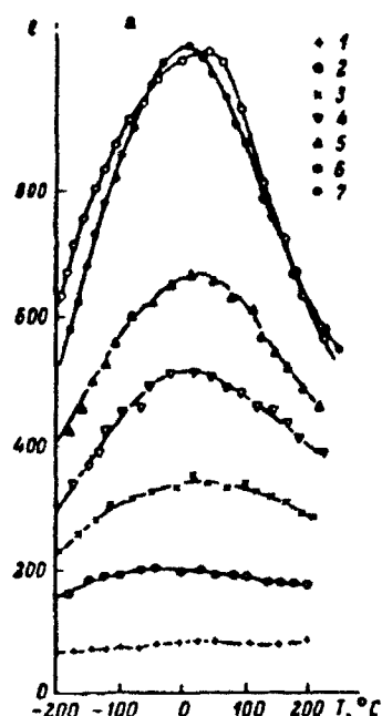
Figure 36.4. Temperature dependences of \epsilon (a) and \tan \delta (b) for (\text{Ba}, \text{Sr})\text{TiO}_3 films. Film thickness d (micrometers): (1) 0.1; (2) 0.33; (3) 0.5; (4) 1.0; (5) 2.0; (6) 5.0; (7) 8.2. Data from Ref. [52].
