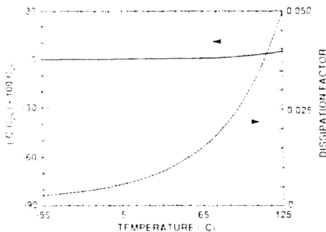
Fig. 6. Change in capacitance with respect to the capacitance and dissipation factor at 1 kHz vs. temperature at 1 kHz for the disk barrier layer capacitor of composition BHP.
