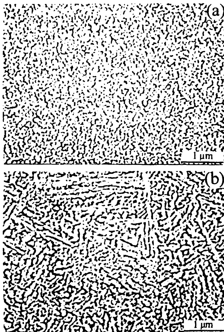
FIGURE 4. SEM micrographs of \text{La}_2\text{Ti}_2\text{O}_7 thin films on (a) fused silica and (b) Si(100) heat treated at 800^\circ\text{C} for 1 h.
