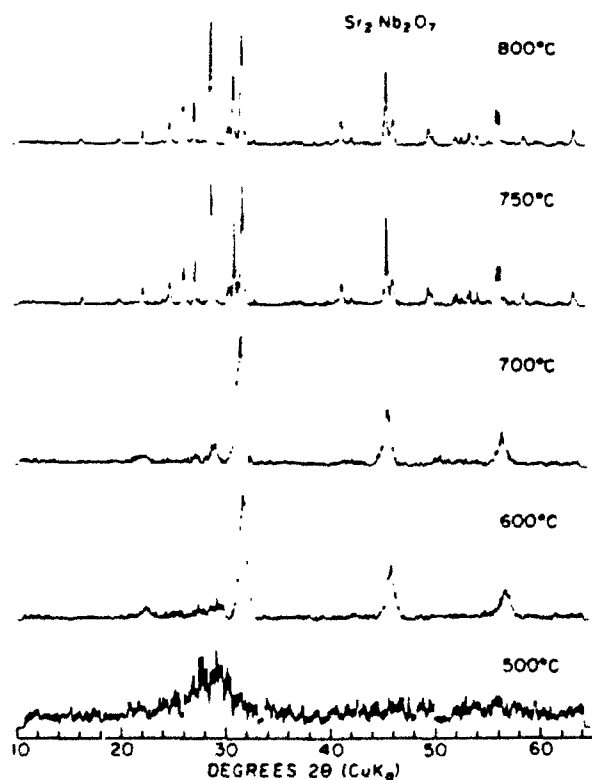
Fig. 3. XRD patterns of \text{SrNb}_2\text{O}_7 gel powder heat-treated at different temperatures.
