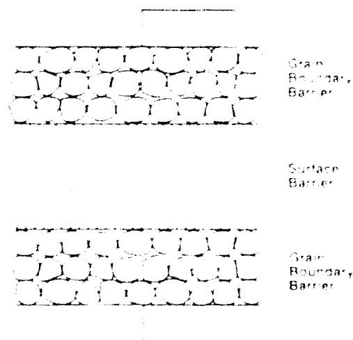
Fig. 8. Schematic diagram of a grain boundary barrier layer capacitor of BHP.
