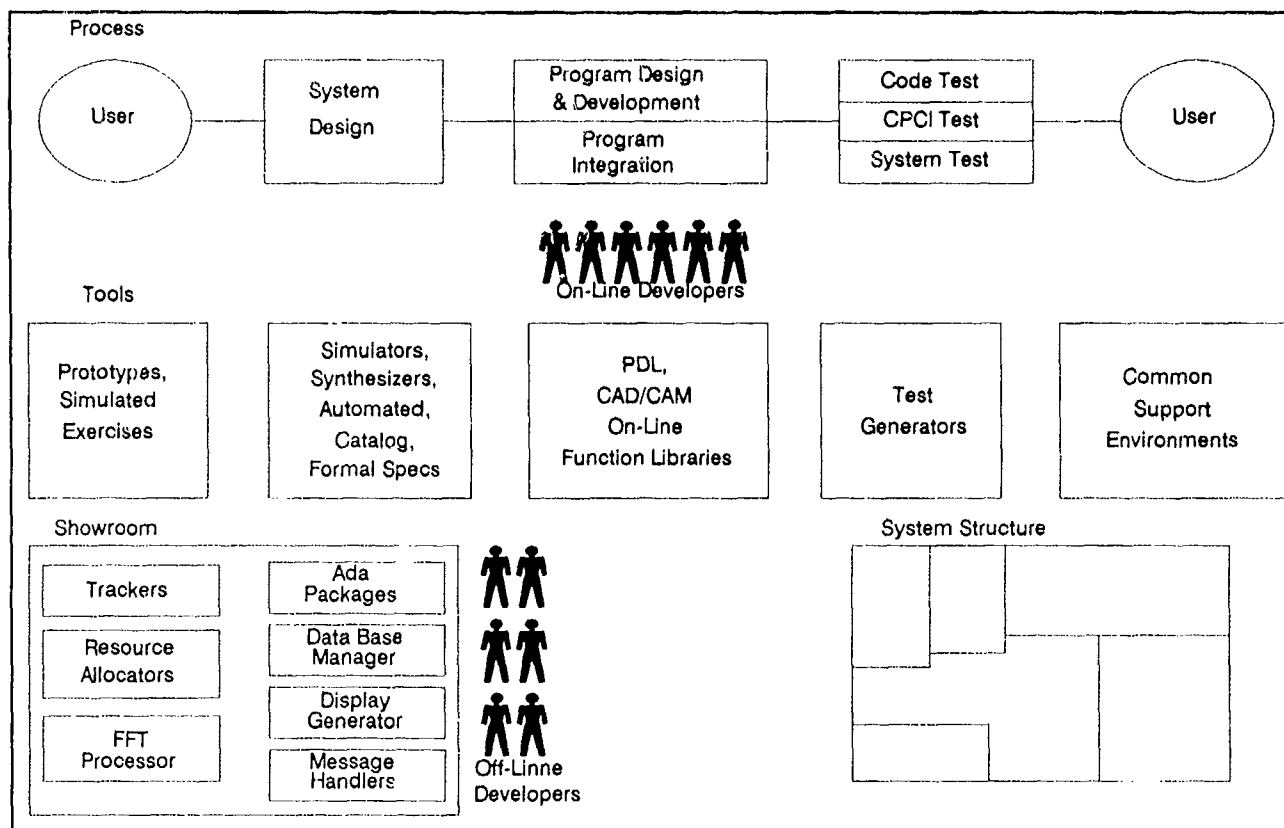
Fig. 13-2 Reusability
