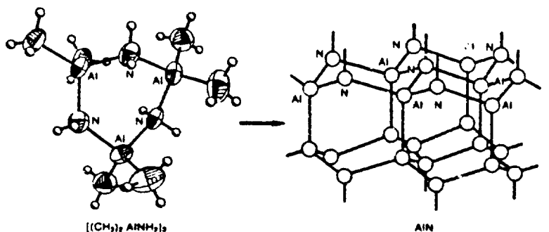
Fig. 3. Structural relationship between [\text{Me}_2\text{AlNH}_2]_3 and \text{AlN} .
