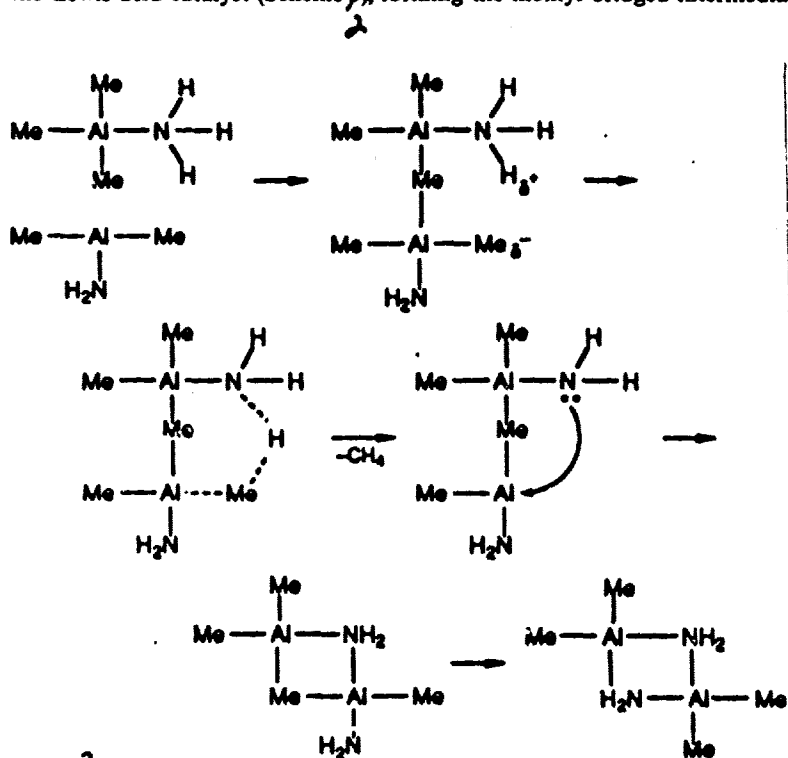
Scheme 2. Proposed mechanism for the thermal decomposition of \text{Me}_3\text{AlNH}_2 .
