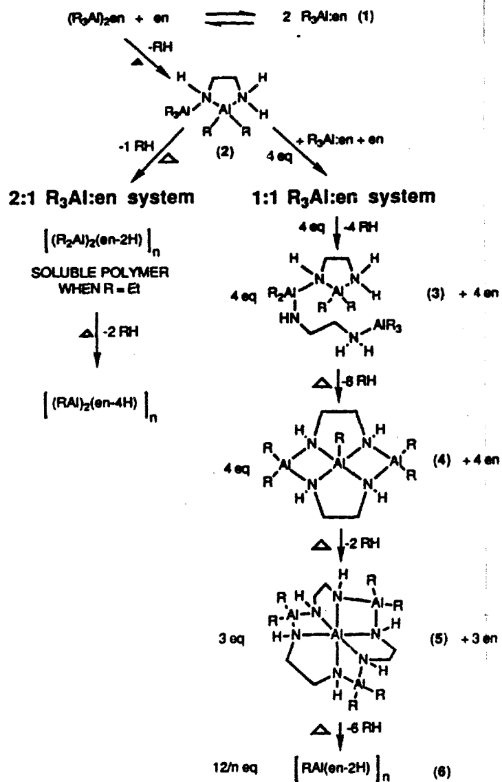
Scheme 1. Suggested pathways for the thermal decomposition of the (R_3Al)_n adducts.
