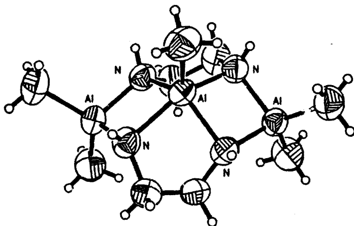
Fig. 4. Ortep plot of the \text{MeAl}[(\text{HNCH}_2\text{CH}_2\text{NH})\text{AlMe}_2]_2 structure.
