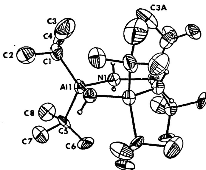
Fig. 2. Ortep plot of (i\text{-Bu})_3\text{AlNH}_2 . Hydrogen atoms omitted (except on N) for clarity.
