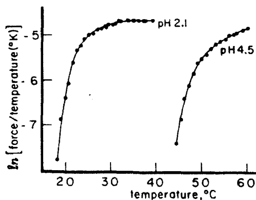
Figure 1. Thermomechanical transduction exhibited by X 20 -poly[4(VPGVG)(VPGE)]. At pH 2.1 contraction begins on raising the temperature from just below 20°C and is completed just above 30°C. At pH 4.5 contraction does not begin until above 40°C and is completed just above 60°C. (Reproduced with permission from reference 4).
