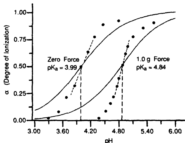
Figure 2. When X^{20} -poly[4(VPGVG), (VPGEg)] is titrated without force being applied to the elastomer, an acid base titration curve is obtained with a pK_a of 3.99. After the elastomer has been stretched by the application of a force, the pK_a is raised, in this study, to 4.84 and the steepness of the curve is increased. See text for discussion. (Reproduced with permission from reference 5).
