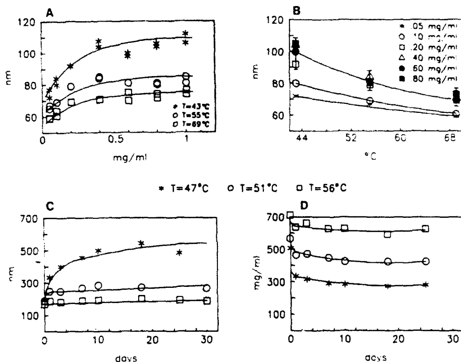
Figure 5. Concentration, temperature and time dependence for nanoparticles formed from poly(VPGVG). Recognizing that the ordinates are given as radii, particle diameters from 100 to 1000 nm are observed. (Reproduced from reference 21 with permission).
