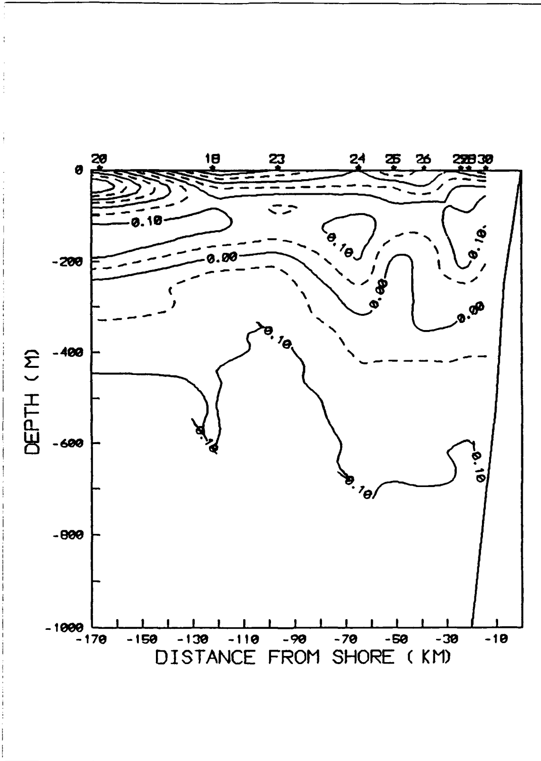
Figure 13 Spiciness for the Canyon Section (contour interval of 0.05)
