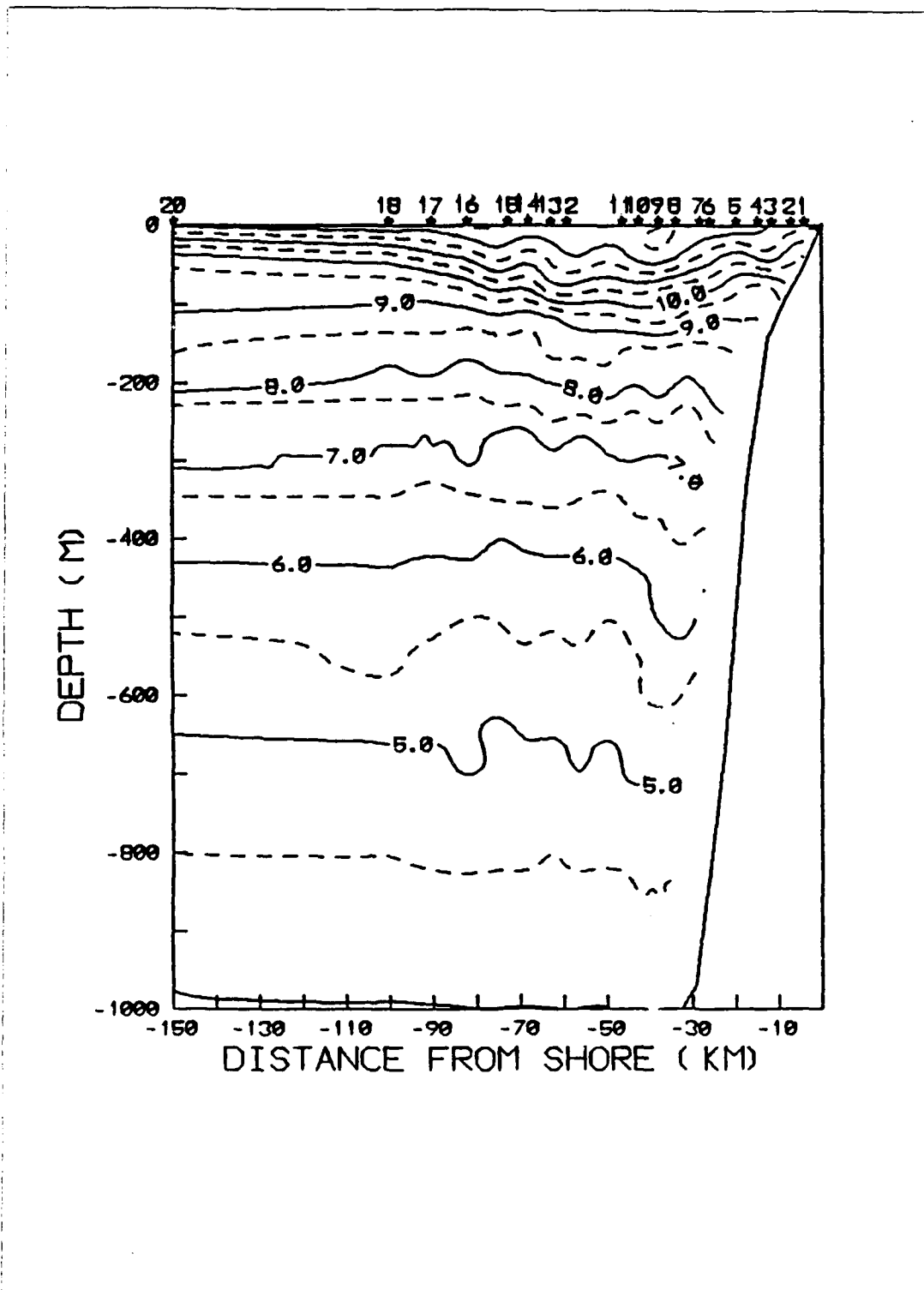
Figure 6 Temperature for the Pt. Sur Section (contour interval of 0.5 °C)
