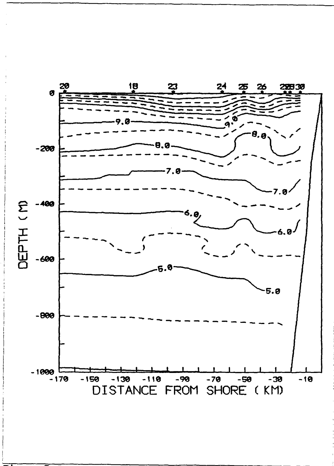
Figure 7 Temperature for the Canyon Section (contour interval of 0.5 °C)
