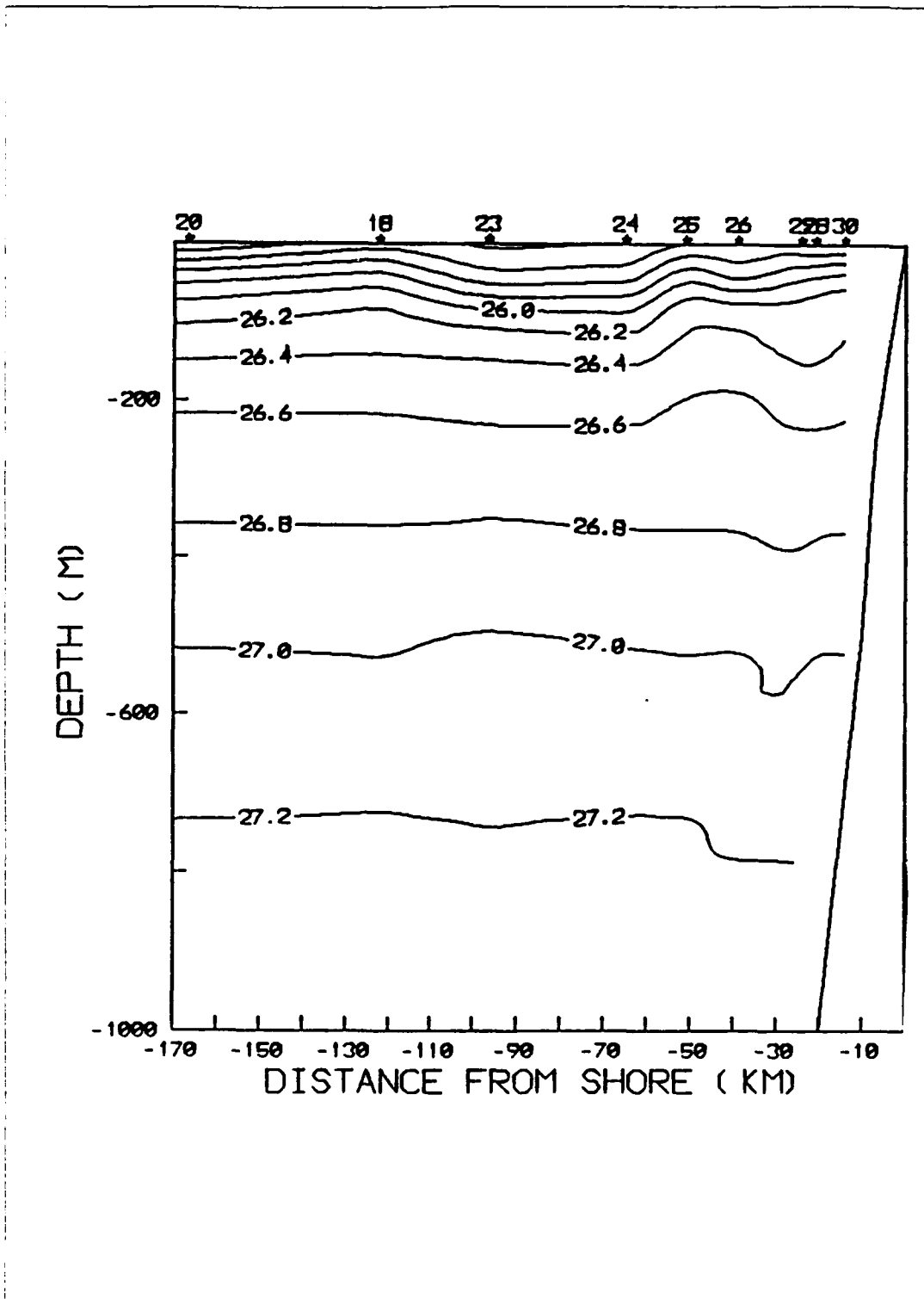
Figure 11 Density ( \gamma ) for the Canyon section (contour interval of 0.2 kg/m 3 )
