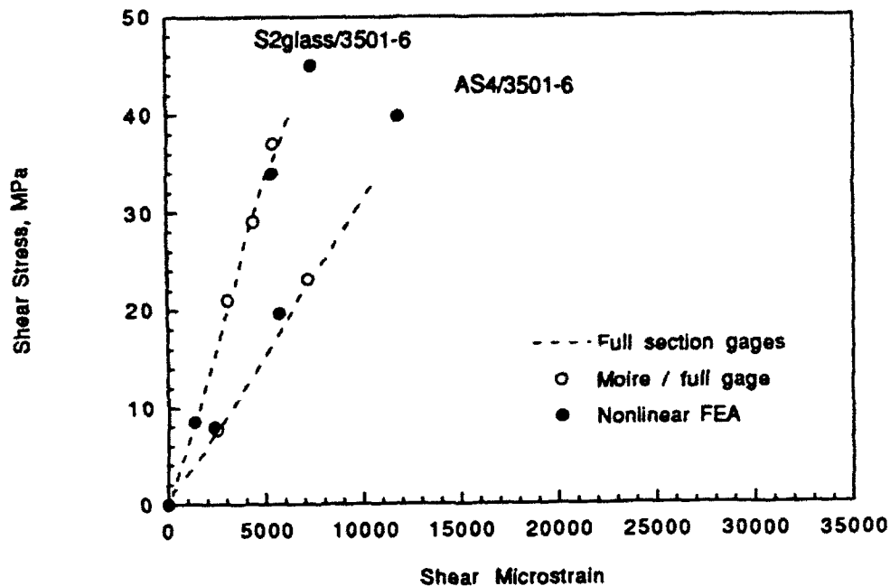
Figure 22 Average shear stress-strain response for AS4/3501-6 and S2 glass/3501-6 unidirectional (G 23 ) specimens measured with moiré interferometry and full section gages vs. predicted values based on finite element analyses with nonlinear elastic material properties
