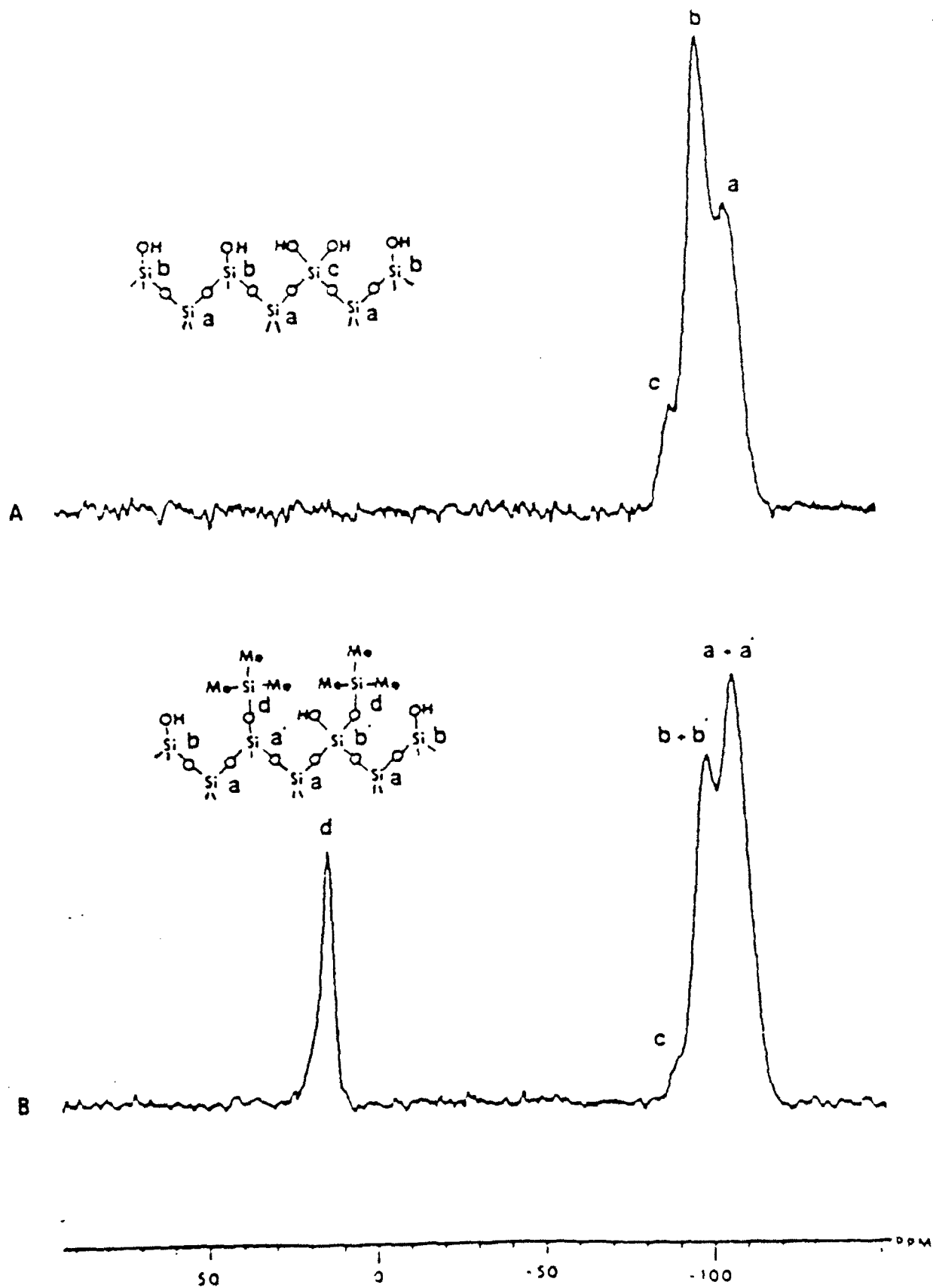
Figure 9. ^{29}\text{Si} CP-MAS spectra of A) silica gel and B) the product of its reaction with trimethylchlorosilane. Reprinted with permission from reference 158, copyright 1982, American Chemical Society.
