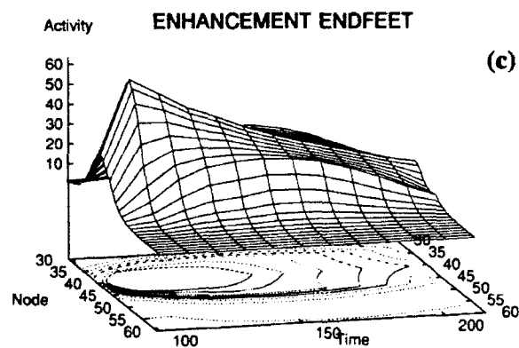
Figure 20. Equidistant split. Activity distributed (a) on glial input endfeet, (b) within interglial layer, (c) on glial enhancement endfeet, and (d) after CE processing. Both the CE activity maxima and the activity edges support the percept of the central stimulus fissioning and moving off toward the two introduced stimuli. Three activity maxima result (instead of two, as is perceived), corresponding to the location of the stimuli in motion. Eventually, the three maxima are replaced by one central maximum, resulting from the separate activity "mountains" merging.
