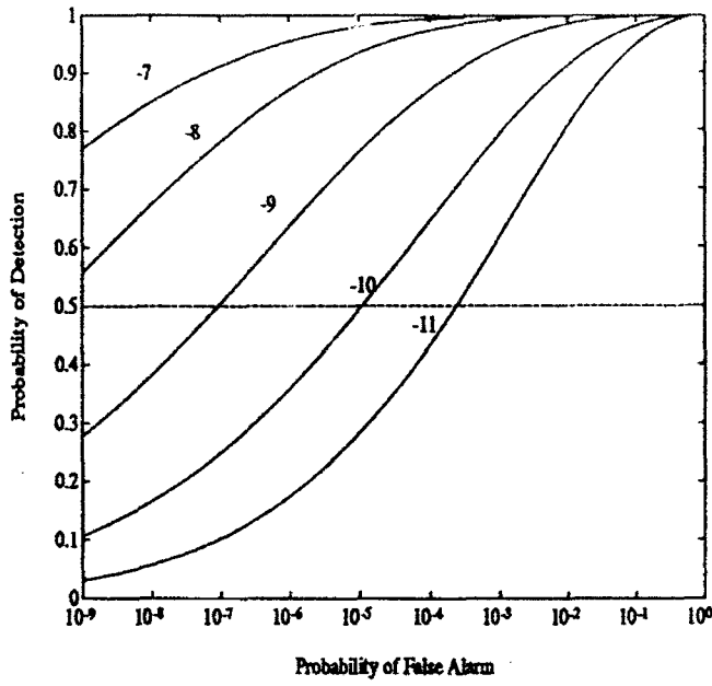
Figure 5: Semi-empirical Receiver Operating Characteristic Curves Using Johnson Distributions for the Sigmoided Outputs Indexed by Signal Level Offsets (in dB).
