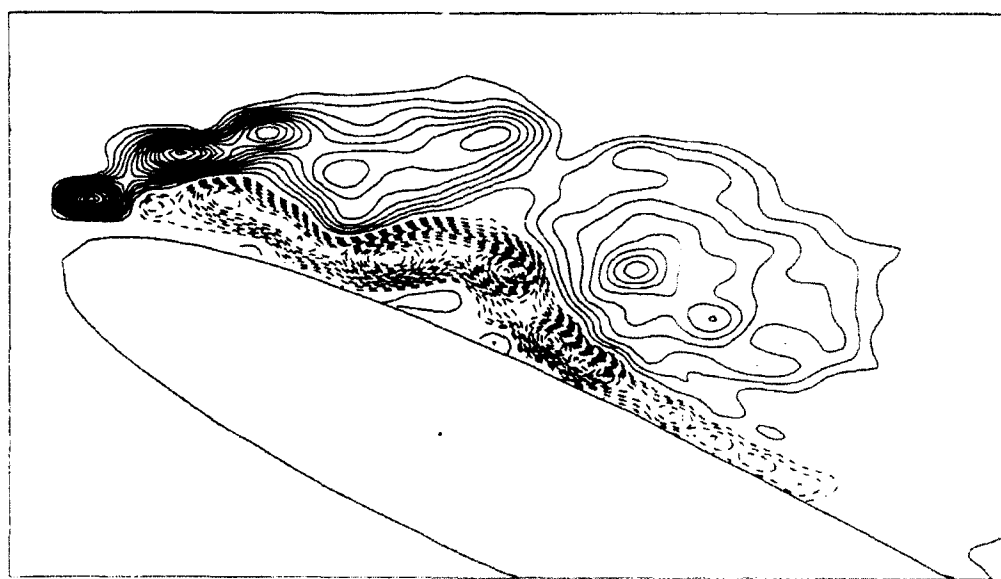
Instantaneous Vorticity
