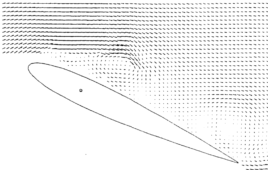
Instantaneous Velocity
