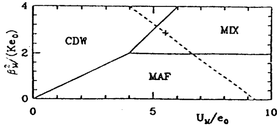
FIG. 1. t_0=0 phase diagram of an infinite chain for \beta_X/\beta_M=-1 , U_X/U_M=1 . The dashed line is the parameter path used for Fig. 4 and + the point in Fig. 3. Note that changing P is equivalent to moving along a line through the origin.
