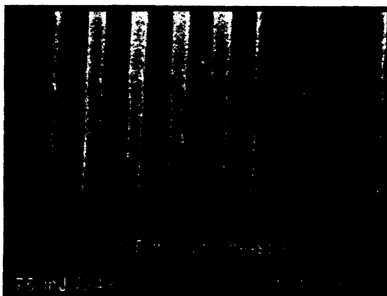
Figure 5: Positive tone image obtained with polymer 11 in a dry develop process (resist formulation see experimental section, post apply bake 2 min at 110^\circ\text{C} , 75 \text{ mJ}/\text{cm}^2 projection print, PEB 12 min at 125^\circ\text{C} , gas-phase silylation with \text{Me}_2\text{NSiMe}_3 for 75 sec, \text{O}_2 -RIE ( 0.5 \text{ kW} , 6 torr, 10 sccm, 1.3 min)).
