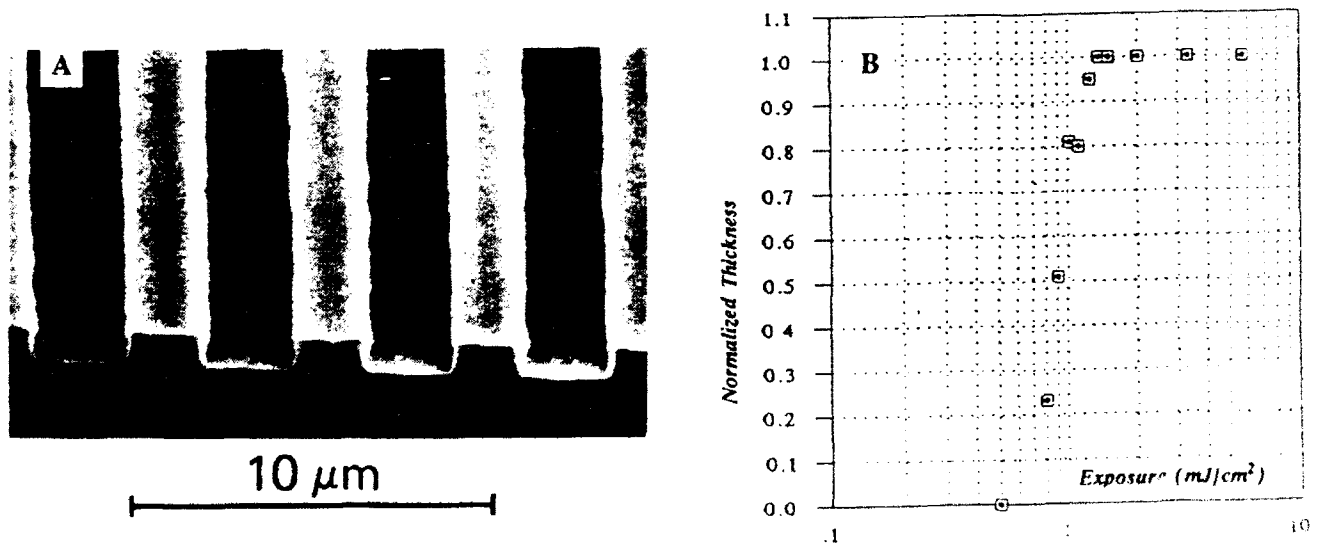
Figure 3: a) Scanning electron micrograph of a negative tone image obtained from carboxylic acid polymer 11 with photo-base generator 10. (1 μm resist prebaked at 110°C for 2 min, exposed to 33 mJ/cm² at 254 nm (contact print), postbaked at 125°C for 14 min; developed by soaking in water for 30 sec and treating with an aqueous solution of triethanolamine (2.3 g/l) for 12 sec.) b) Contrast curve for the wet develop process.
