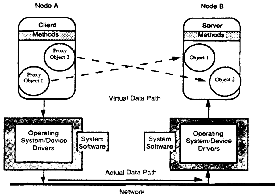
Figure 13: A Schematic Representation of Proxy Objects
