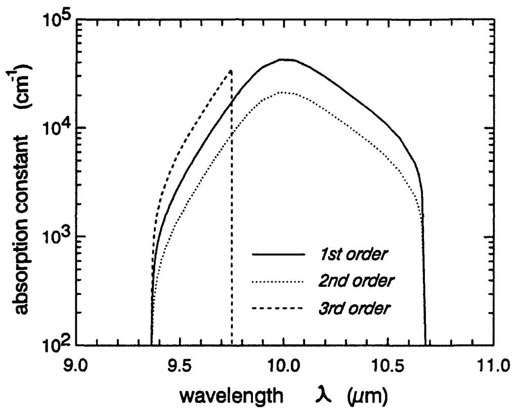
Figure 3.5.5 (a) Optical absorption constant of the 1st, 2nd, and 3rd order diffracted waves vs. wavelength for a 2-D square mesh grating coupled GaAs/AlGaAs QWIP.
