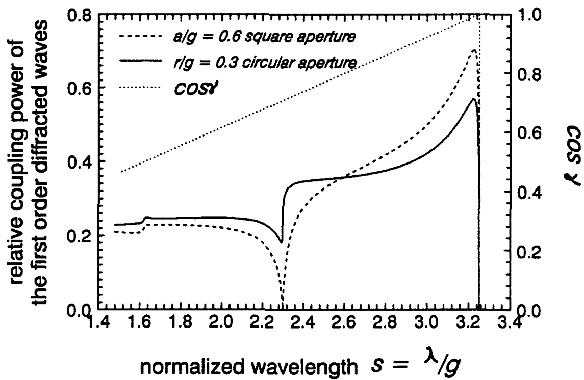
Figure 3.5.3 (b) The relative coupling power of the 1st order diffracted waves vs. normalized wavelength for a square and circular shape aperture.
