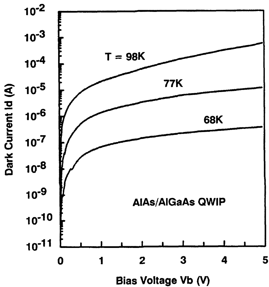
Figure 3.3.3 Dark current versus bias voltage for the AlAs/AlGaAs QWIP measured at 98, 77 and 68 K.
