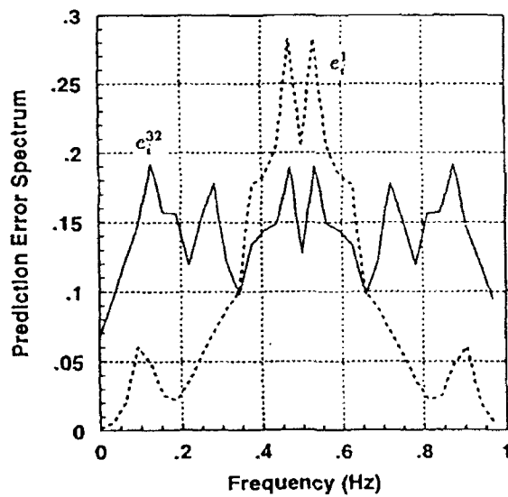
Figure 4: Estimated Spectrums of Prediction Errors
