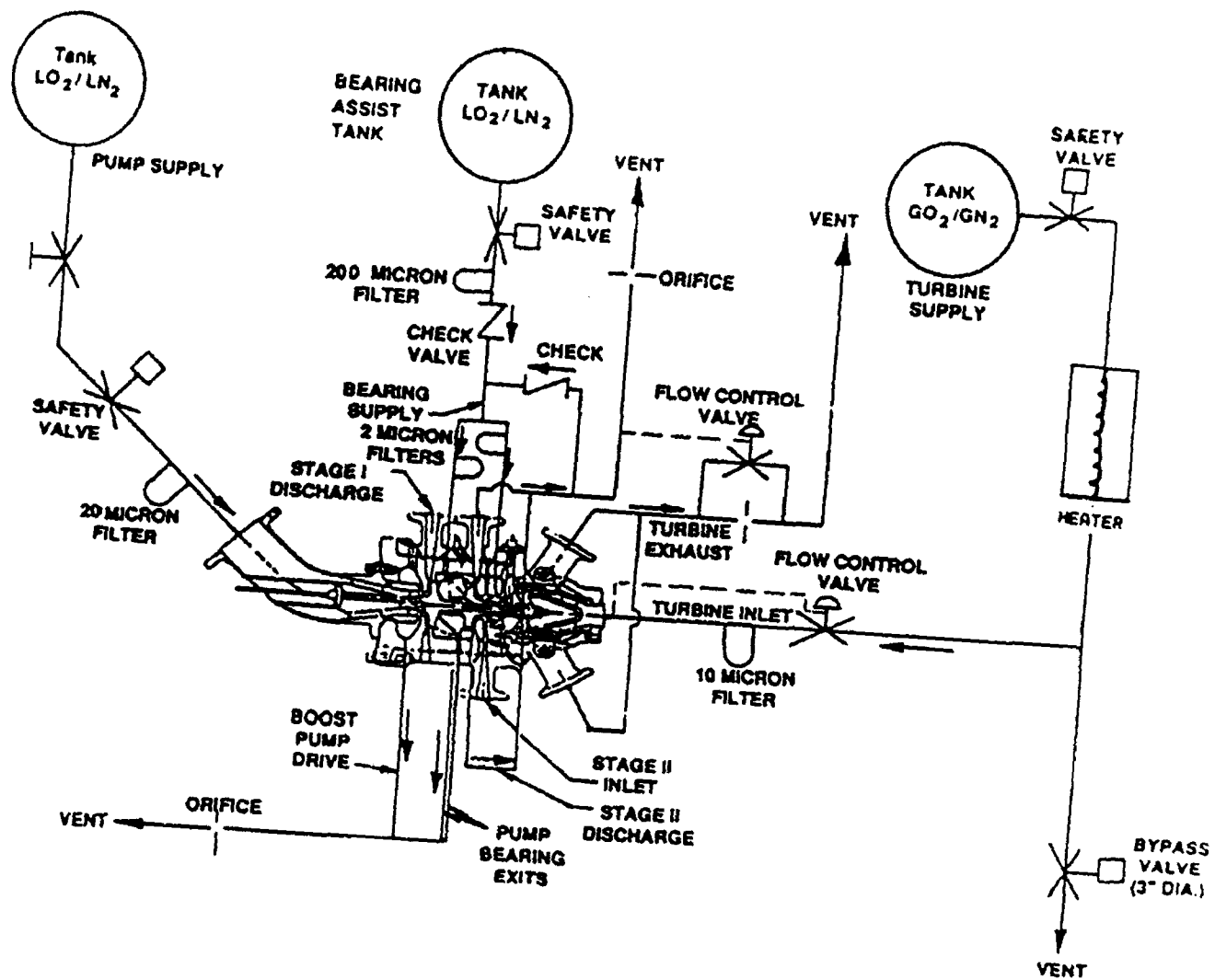
Figure 4. Test Schematic Series F and G
