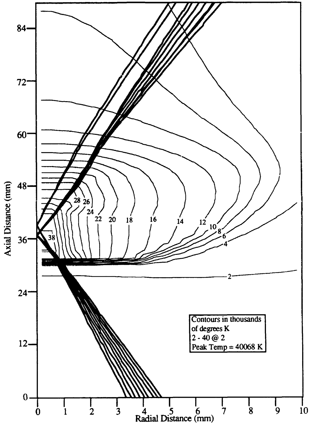
Figure 5.14 Electron temperature contours of the core region of case tf45, which is a 70kW, 3.5 atm, f-4, 2192.9 gmoles/m 2 s hydrogen LSP.
