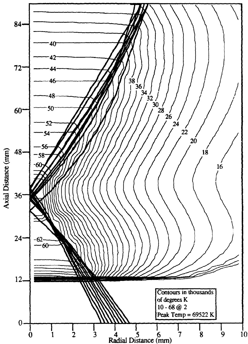
Figure 5.15 Electron temperature contours of the core region of case f5, which is a 700kW, 3.5 atm, f-4, 2192.9 gmol/m 2 s hydrogen LSP.
