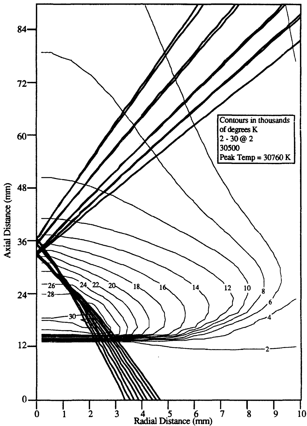
Figure 5.2 Electron temperature contours and beam ray trace for the core region of case tf37 which is a 70kW, f-4, 3.5 atm, 2192.9 moles/m 2 s LSP from a line spark.
