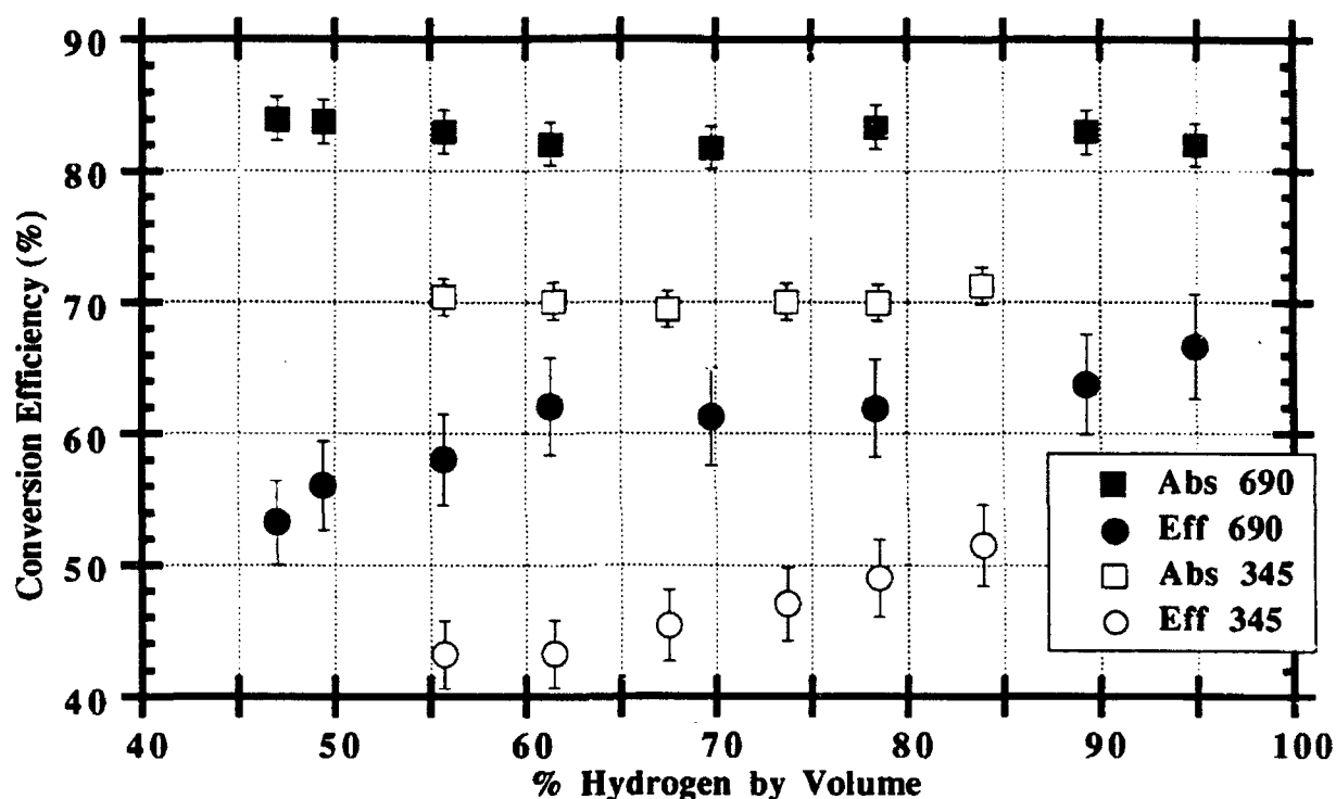
Figure 2.2 Global Absorption and Thermal Efficiency for mixtures of argon and hydrogen at fixed total mole fluxes of 345 moles/m 2 s and 690 moles/m 2 s, 7kW, f-4.1, and approximately 2.5 atm.
