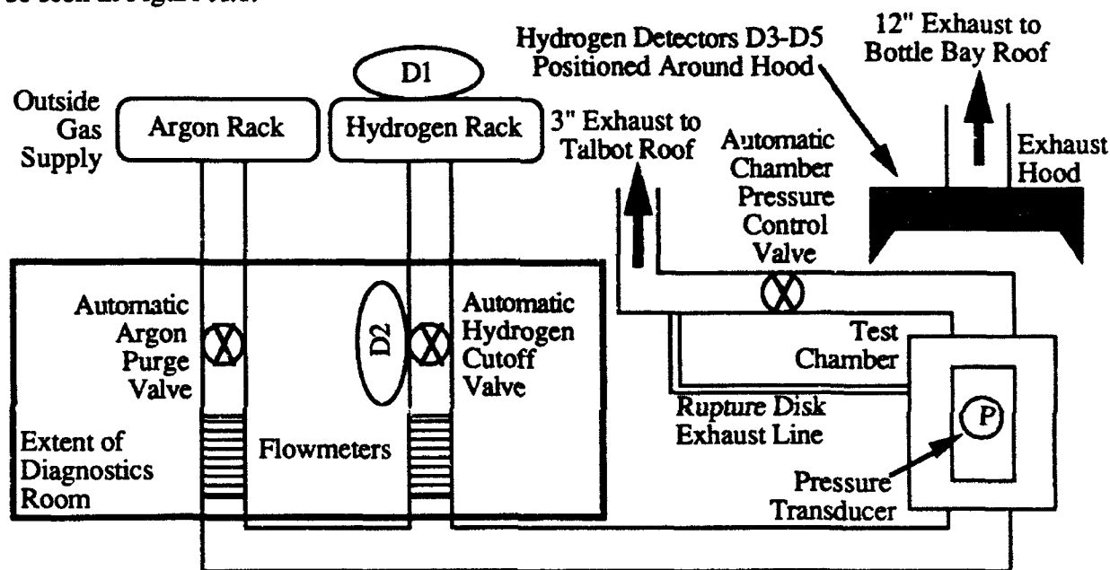
Figure A.1 Diagram of the hydrogen handling and safety system
