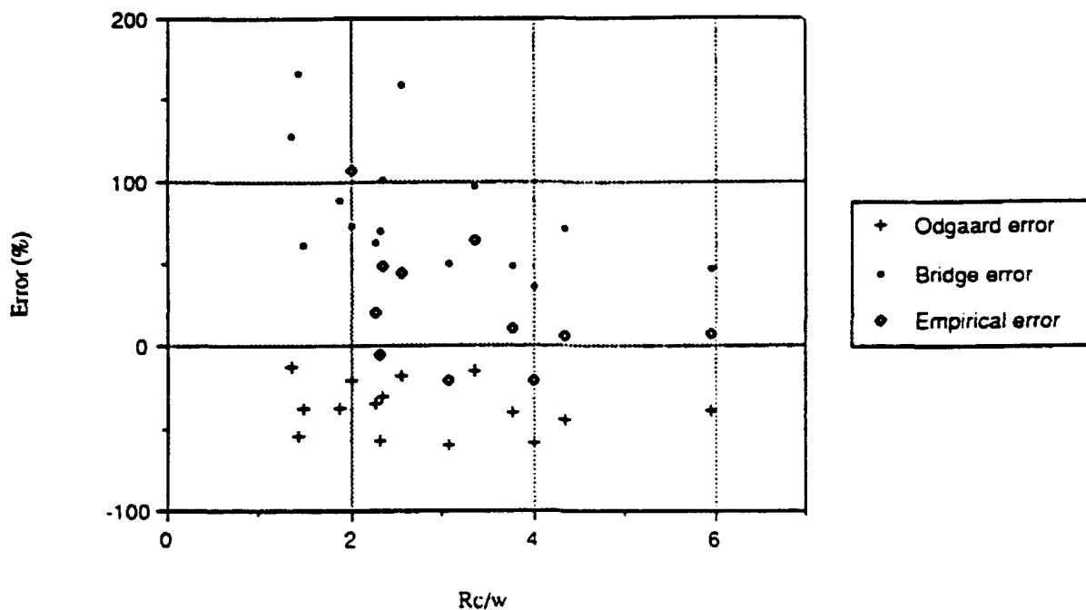
Fig. 17 Errors in Predicted Maximum Bend Scour Depths for data from various researchers
