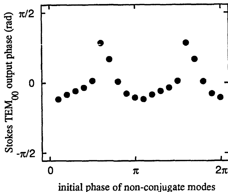
Figure 2.5. Demonstration of the effects of noise modes on the phase of the Stokes mode that is conjugate to the pump. The phase of the initiating radiation was held constant for the \text{TEM}_{00} mode and varied for the phase of the nonconjugate modes.
