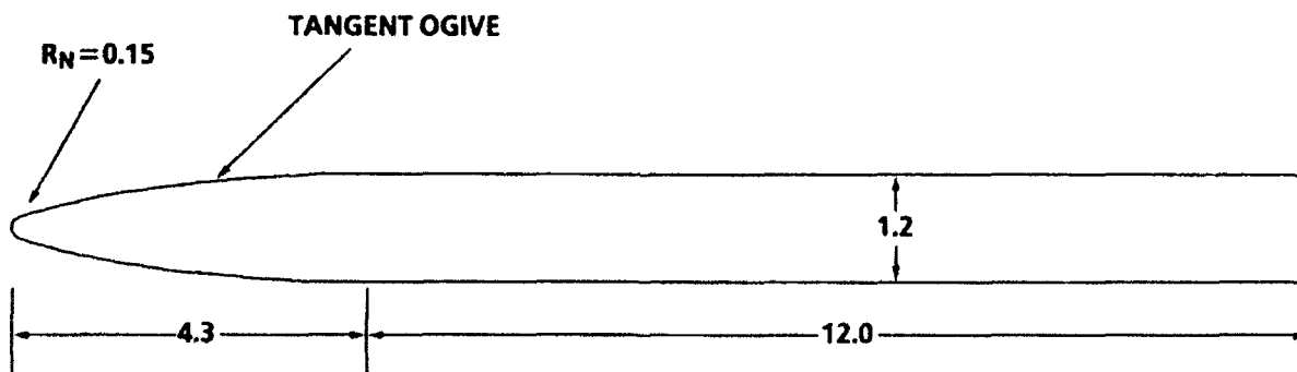
FIGURE 19a. BODY-ALONE CONFIGURATION USED IN VALIDATION PROCESS 31
