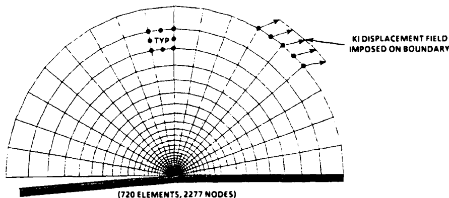
Figure 1. Finite-element mesh for the small-scale yielding computations
