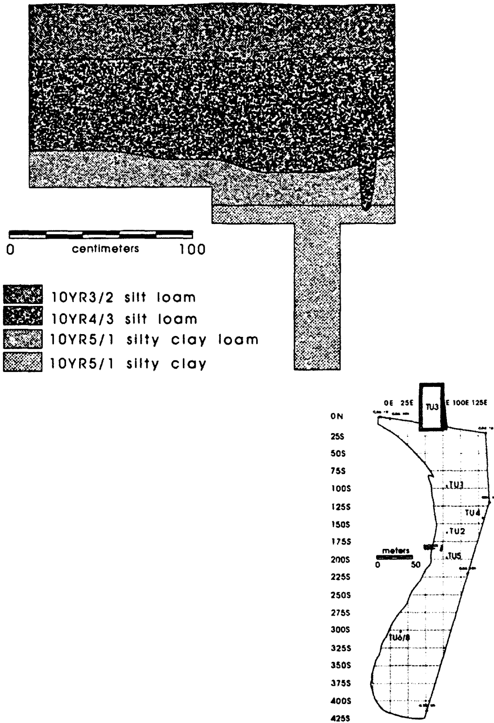
Figure 51. Profile of Test Unit 3 at 23SR1067.
