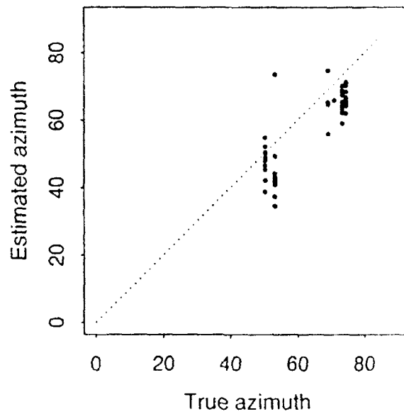
Khibiny, 1-3 Hz, SNR > 3
