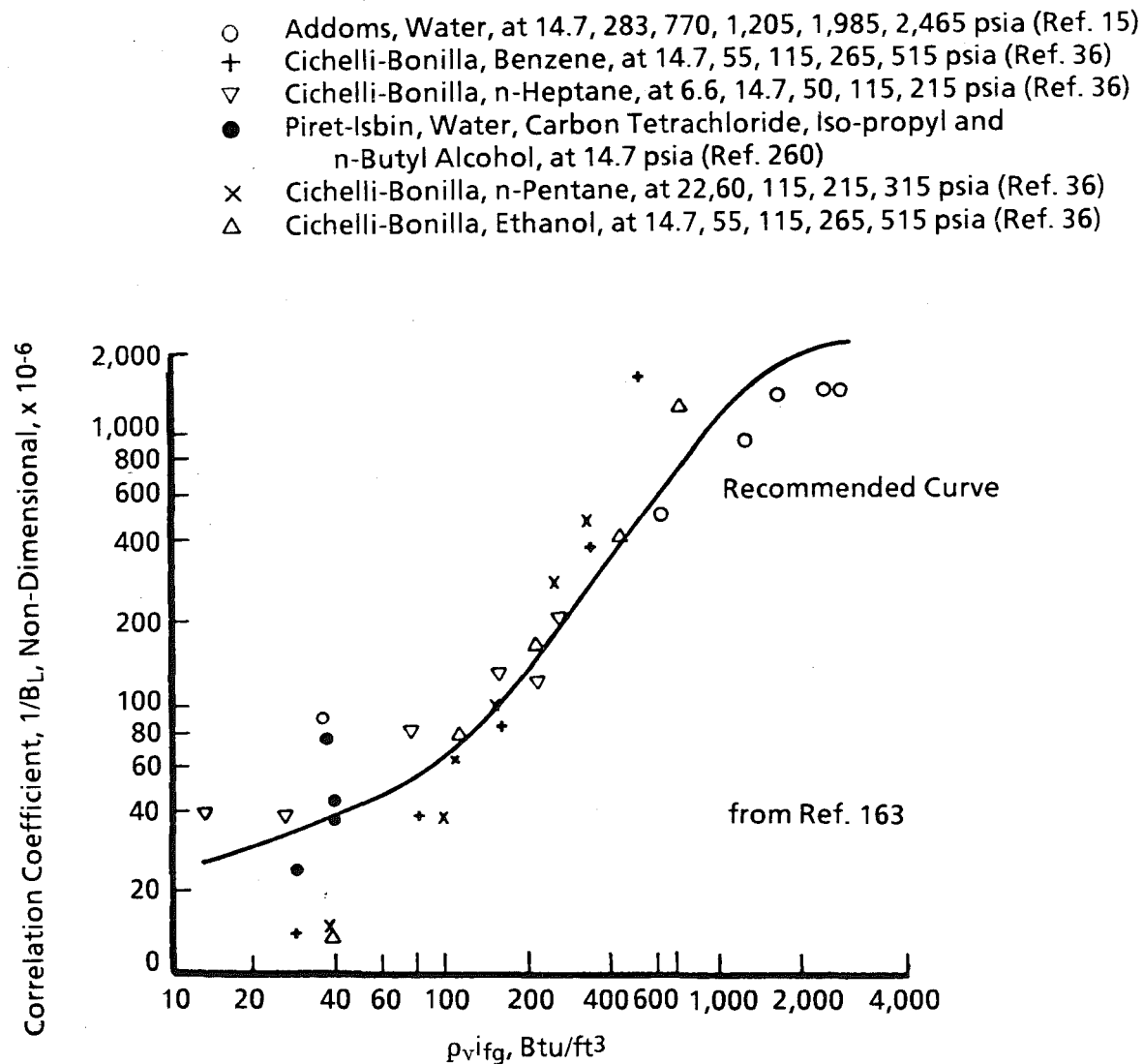
Figure 38. Determination of the coefficient B_L in the Levy correlation.
