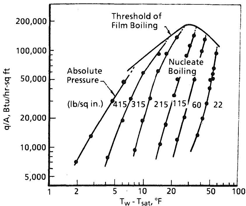
Figure 9. Optimum pressure for the boiling of n-pentane.
