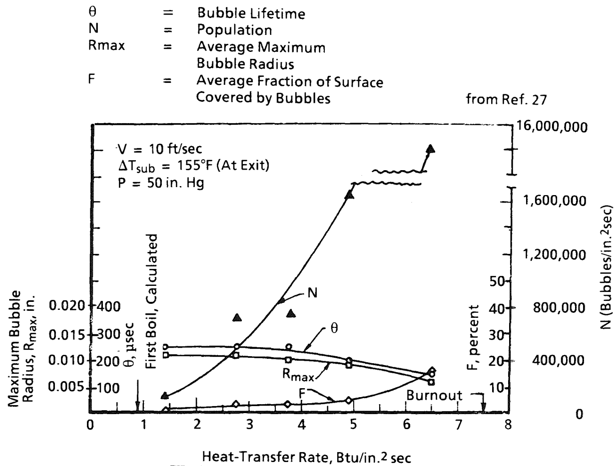
Figure 36. Effect of heat-transfer rate on bubble characteristics.
