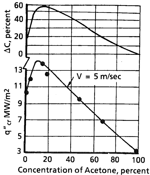
b. Acetone-water
