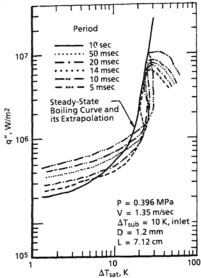
Figure 33. Effect of transient heating on boiling curve.
