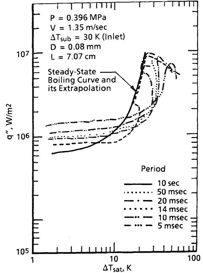
Figure 33. Effect of transient heating on boiling curve.
