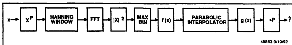
Figure 1. Frequency Estimation Algorithm
