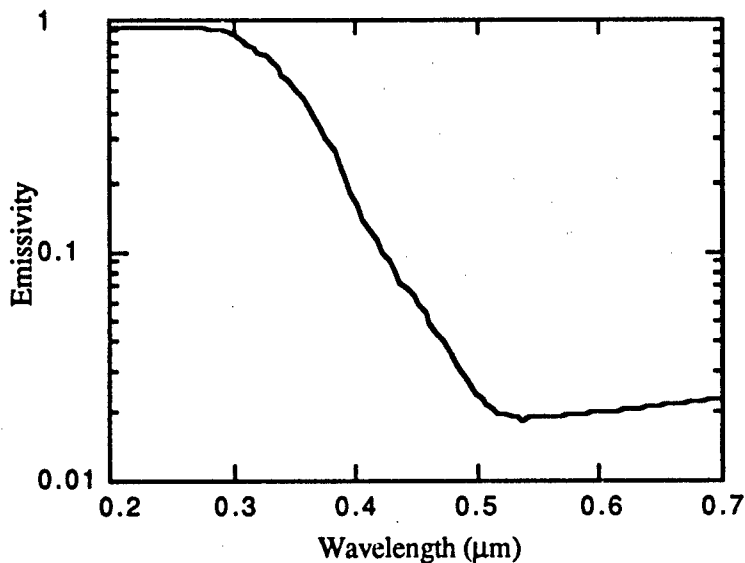
Fig. 13 - An emissivity curve for plume aluminum particles (2.3 \mu\text{m} )
