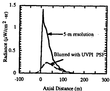
Fig. 28 - CHARM 1.3 predicted and blurred plume axial profile for interval 4
