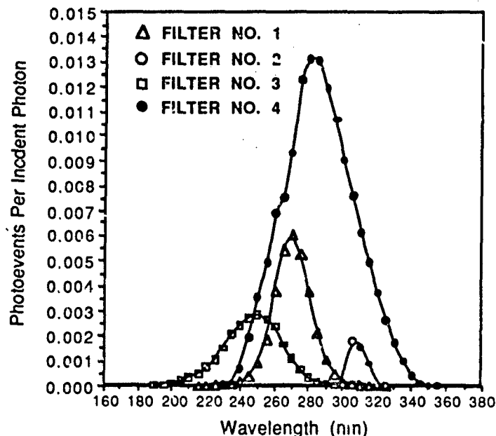
Fig. 2 - Plume camera - net quantum efficiency curves
