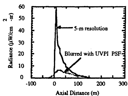
Fig. 25 - CHARM 1.3 predicted and blurred plume axial profile for interval 1
