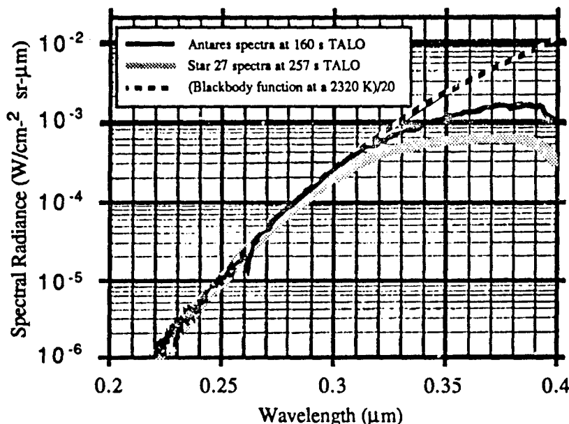
Fig. 15 - On-board spectrometer measurement for Strypi mission
