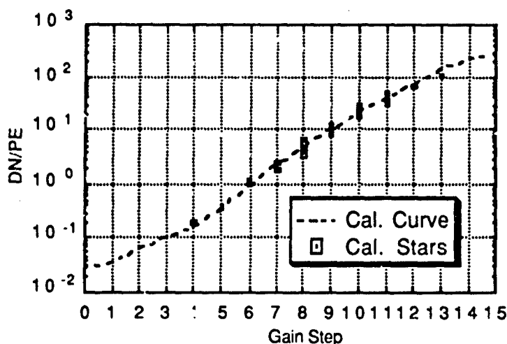
Fig. 7 - Star measurements for plume camera
