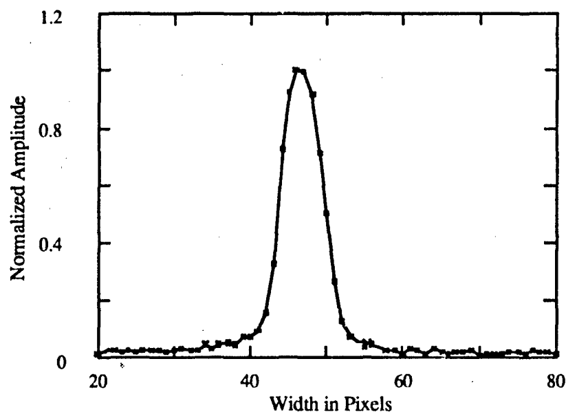
Fig. 18 - Axial profile through plume-camera PSF
