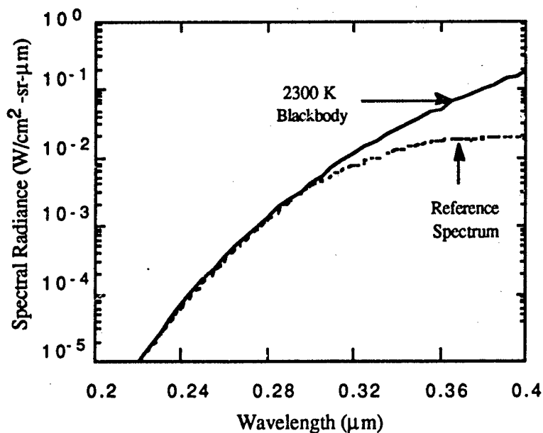
Fig. 14 - Assumed reference spectrum
