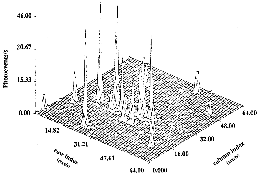
Fig. 10 - Single calibrated plume-camera image of Antares plume
