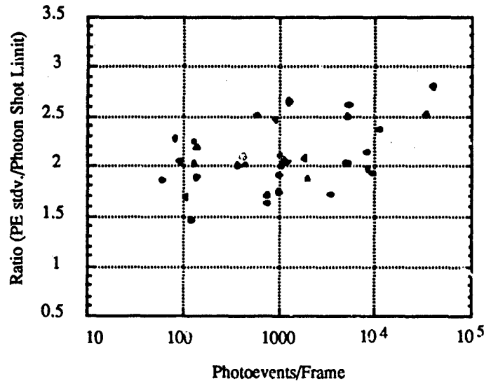
Fig. 34 - Noise in plume-camera star measurements
