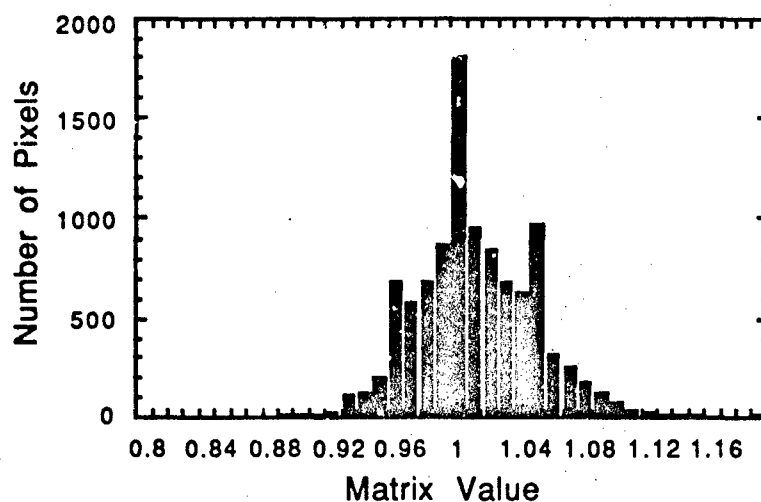
Fig. 5 - Inverse nonuniformity matrix histogram
