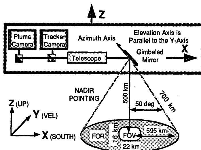
Fig. A8 - Tracker-camera FOV and FOR
