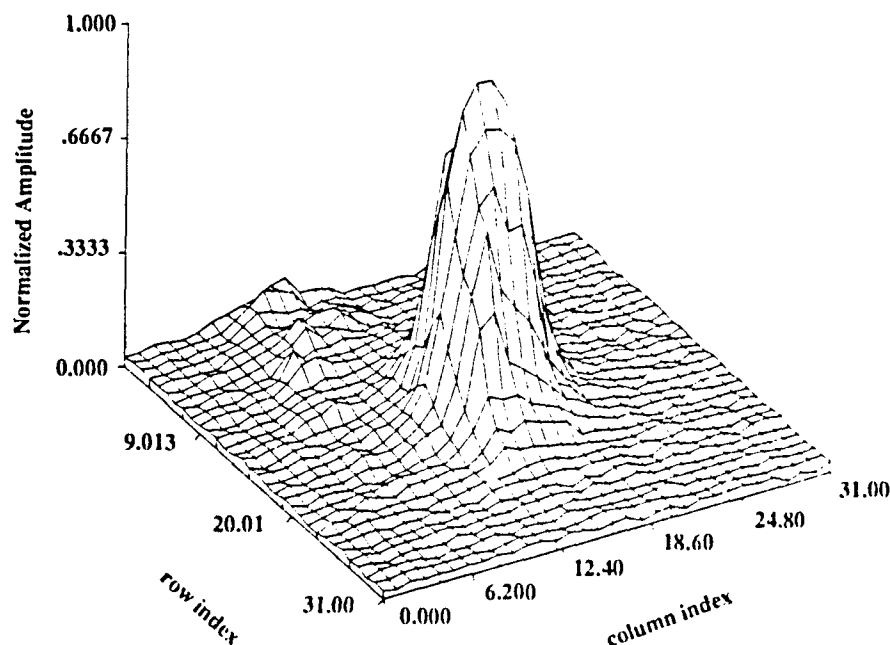
Fig. 17 - Plume-camera PSF for ground-based beacon
