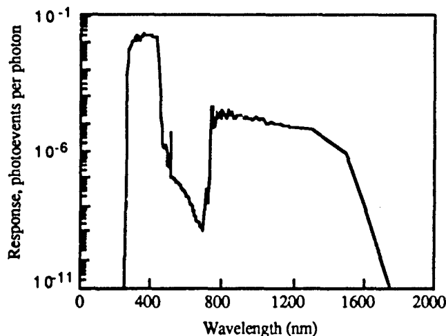
Fig. 33 - Tracker camera - extended net quantum efficiency
