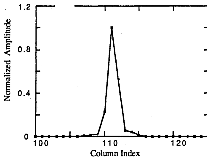
Fig. 21 - Axial profile through tracker-camera PSF
