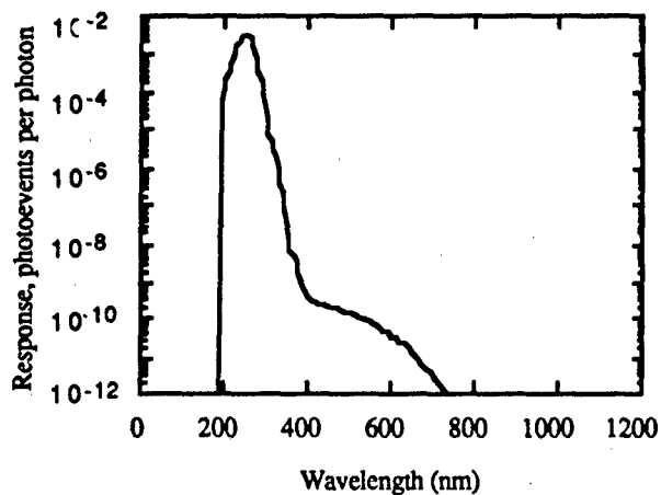
Fig. 31 - Plume camera - extended net quantum efficiency, filter 3
