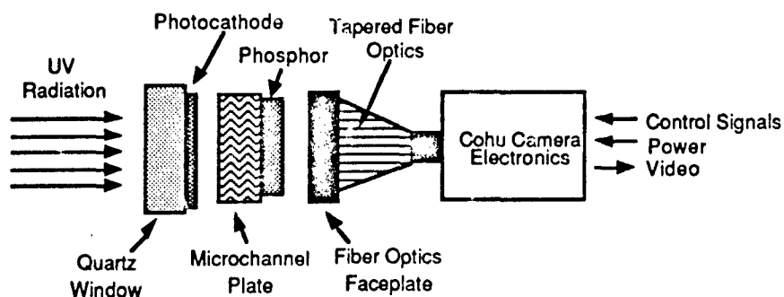
Fig. A4 - UVPI sensor head assembly optics
