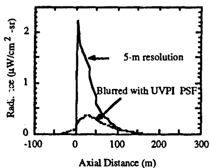
Fig. 27 - CHARM 1.3 predicted and blurred plume axial profile for interval 3
