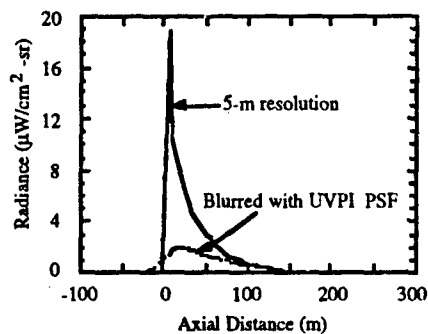
Fig. 26 - CHARM 1.3 predicted and blurred plume axial profile for interval 2
