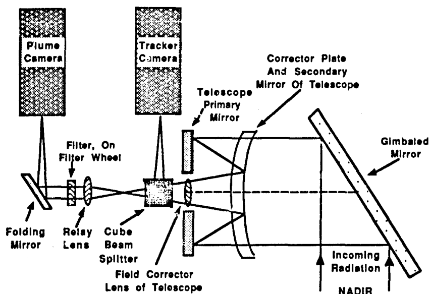
Fig. A4 - UVPI sensor head assembly optics
