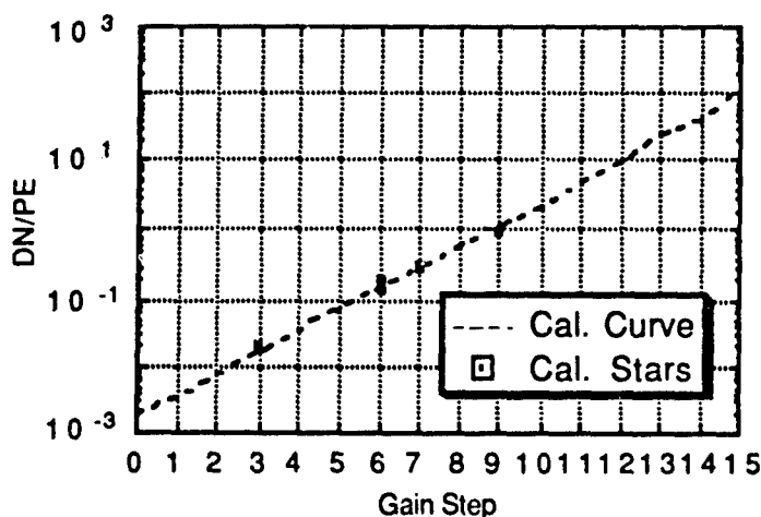
Fig. 8 - Star measurements for tracker camera
