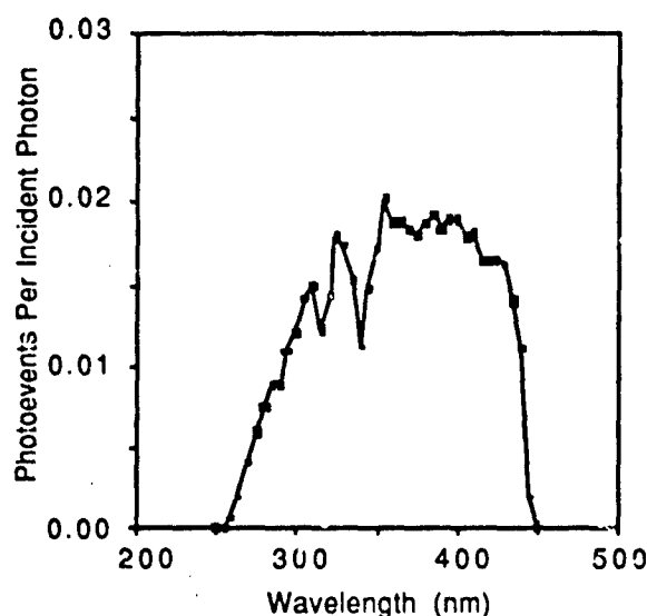
Fig. 3 - Tracker camera - net quantum efficiency curve
