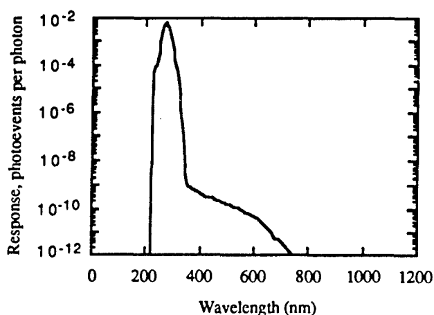
Fig. 29 - Plume camera - extended net quantum efficiency, filter 1
