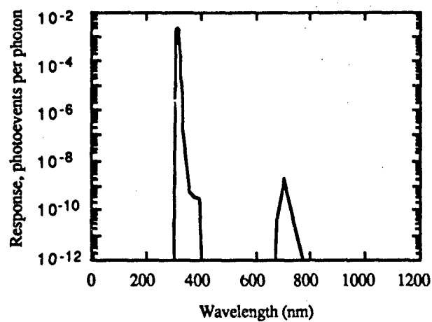
Fig. 30 - Plume camera - extended net quantum efficiency, filter 2
