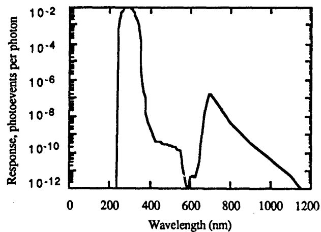
Fig. 32 - Plume camera - extended net quantum efficiency, filter 4
