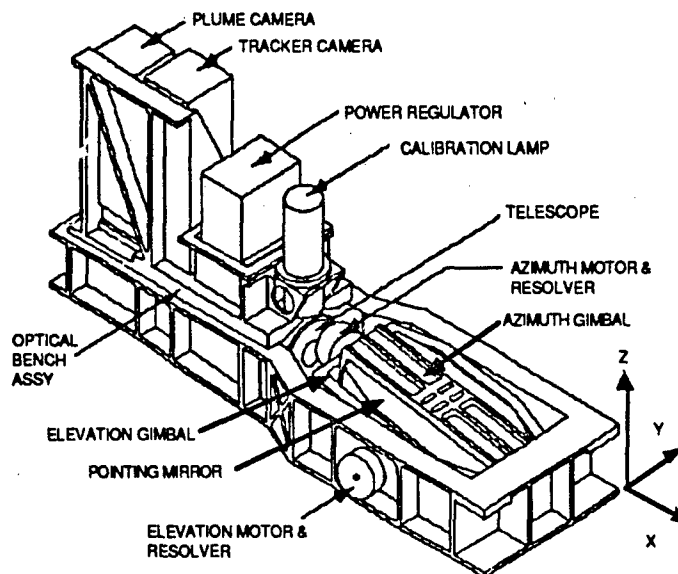
Fig. A3 - UVPI sensor head assembly diagram
