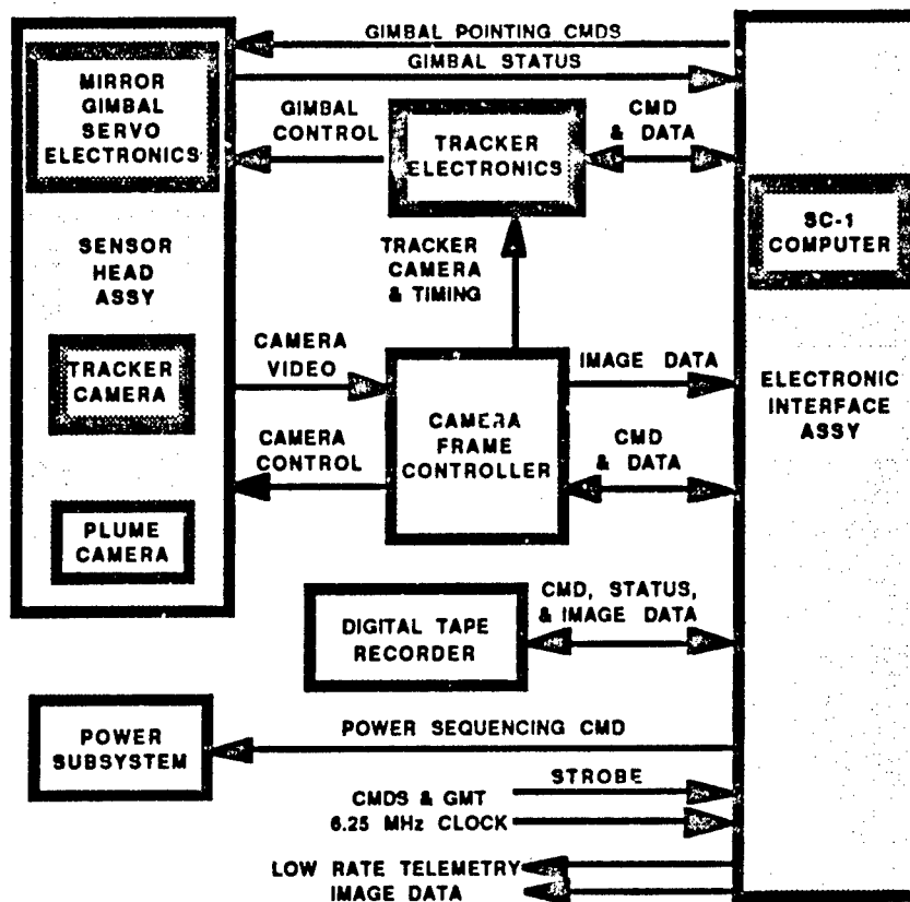
Fig. A2 - Command and data flow within the UVPI
