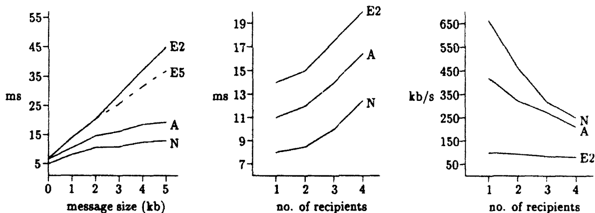
(a) Latency of member-to-group RPC as a function of message size. Group of size of two. (b) Latency of member-to-group RPC as a function of group size. Message of size 1kb. (c) Member-to-group bandwidth as a function of group size.
