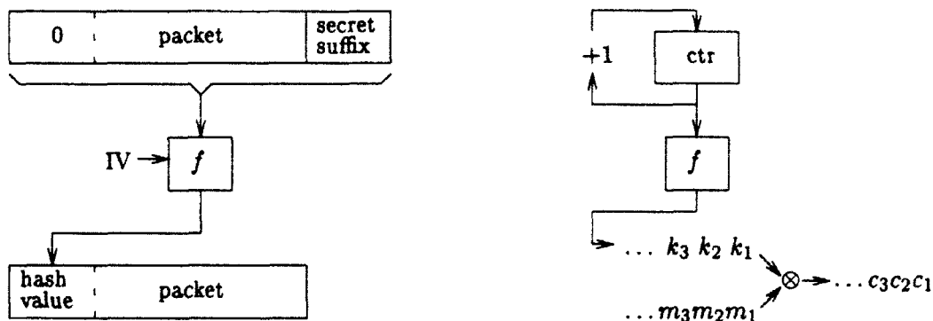
Figure 8: Cryptographic operations
