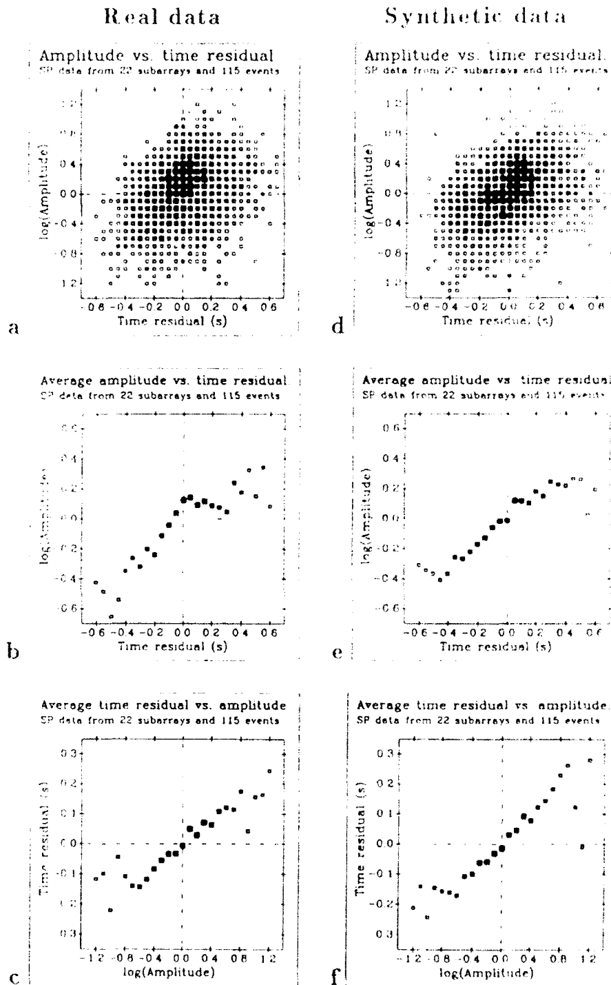
Fig. 2.1.4. (a) Scatter diagram of observed SP peak-to-peak amplitude residual vs time residual for the 22 subarrays and 115 events; (b) Average peak-to-peak amplitudes residual vs binned time residual for the data plotted in (a); (c) Average time residual vs binned amplitude residual for the data plotted in (a); (d,e,f) Same as (a,b,c) but for synthetic data derived from a model for the velocity structure beneath NORSAR.
