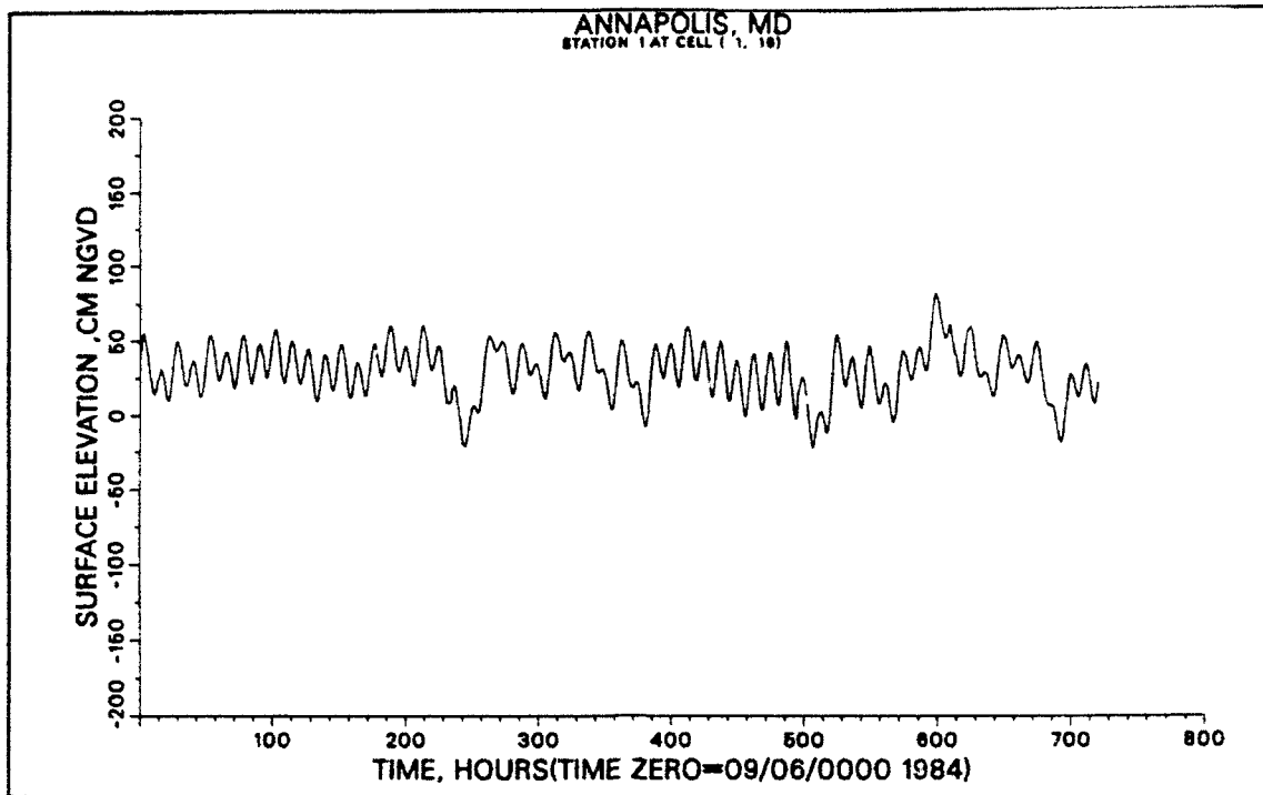
Figure 5a. Recorded tide at Annapolis (hrs)
