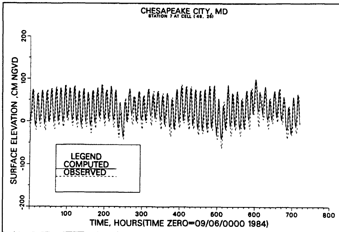
Figure 8d. Computed versus recorded tide at Chesapeake City
