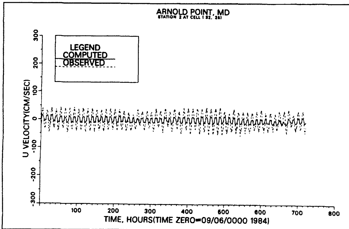
Figure 9d. Computed versus recorded velocity at Arnold Point (4 m)
