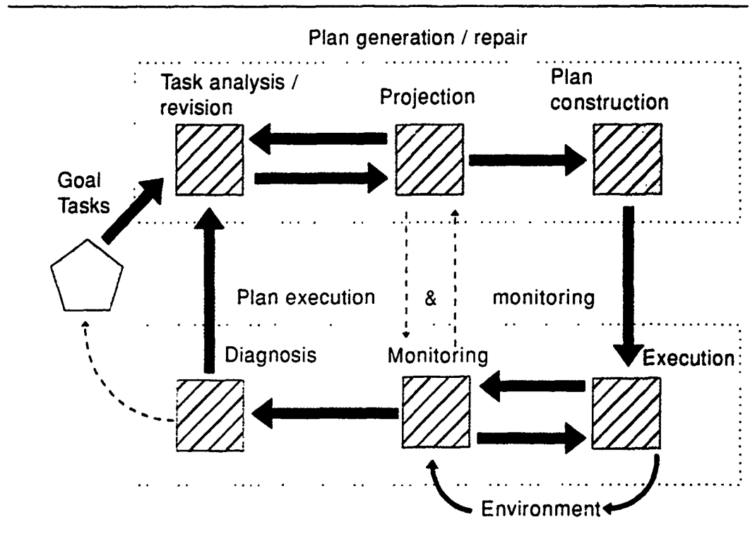
Figure 1.1: The C 2 -planning paradigm.
