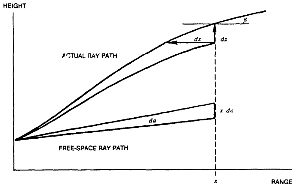
Figure 4. Ray divergence.
