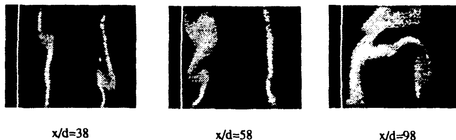
FIGURE 2. Visualizations of OH concentration in a hydrogen diffusion flame at three locations downstream of the nozzle. Reynolds number at the nozzle is Re = 2400 . Nozzle diameter, d = 2.5 mm. Width of the images is x \sim 46 mm in real space.
