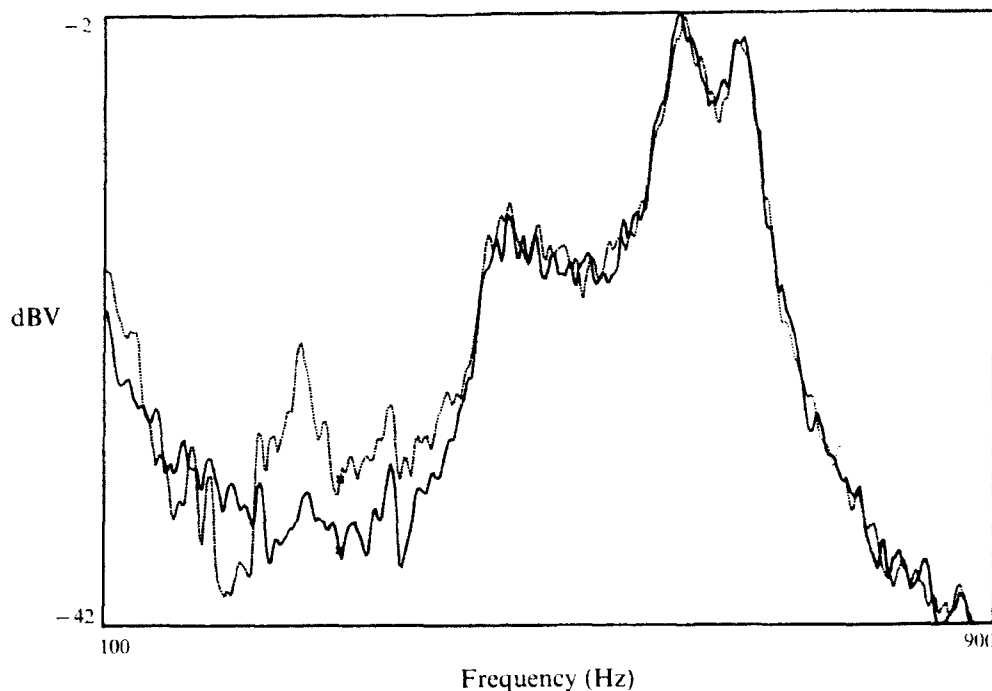
FIGURE 28. Power spectra of u' obtained at different radial locations in the shear layer region: S = 1.00 ; D/\theta = 83 ; x/\theta = 75 ; —, potential core; ---, r = \frac{1}{2}D + 5\theta . The arbitrary reference for the dB scale varies for the two curves.
