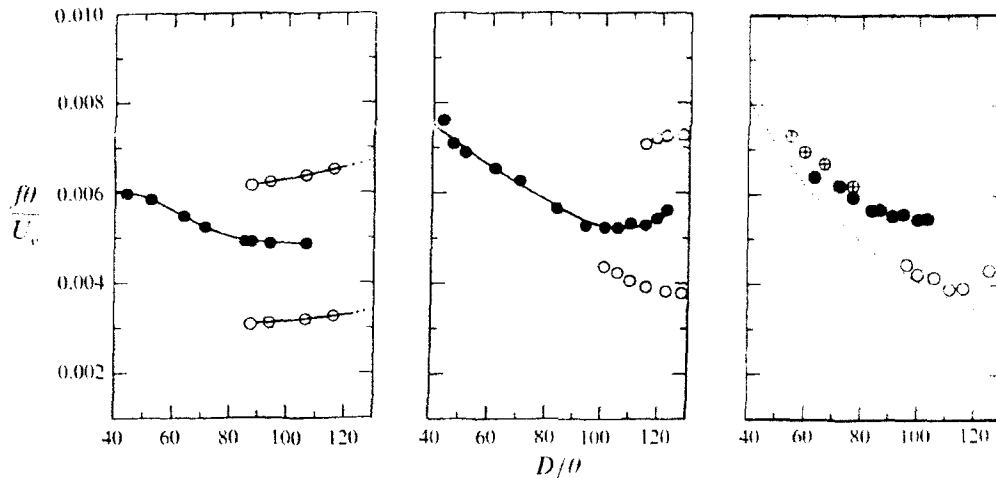
FIGURE 17. Non-dimensional frequency f\theta/U_\infty as a function of D/\theta : x/D = 0.10 ; \bullet , oscillating mode from present experiments: from left to right S = 0.14 , 0.29 and 0.48 respectively. \circ , additional prominent modes in present facility; \oplus , oscillating mode in the heated air jet (Monkewitz et al. 1990); ———, theory (Monkewitz & Sohn 1988).
