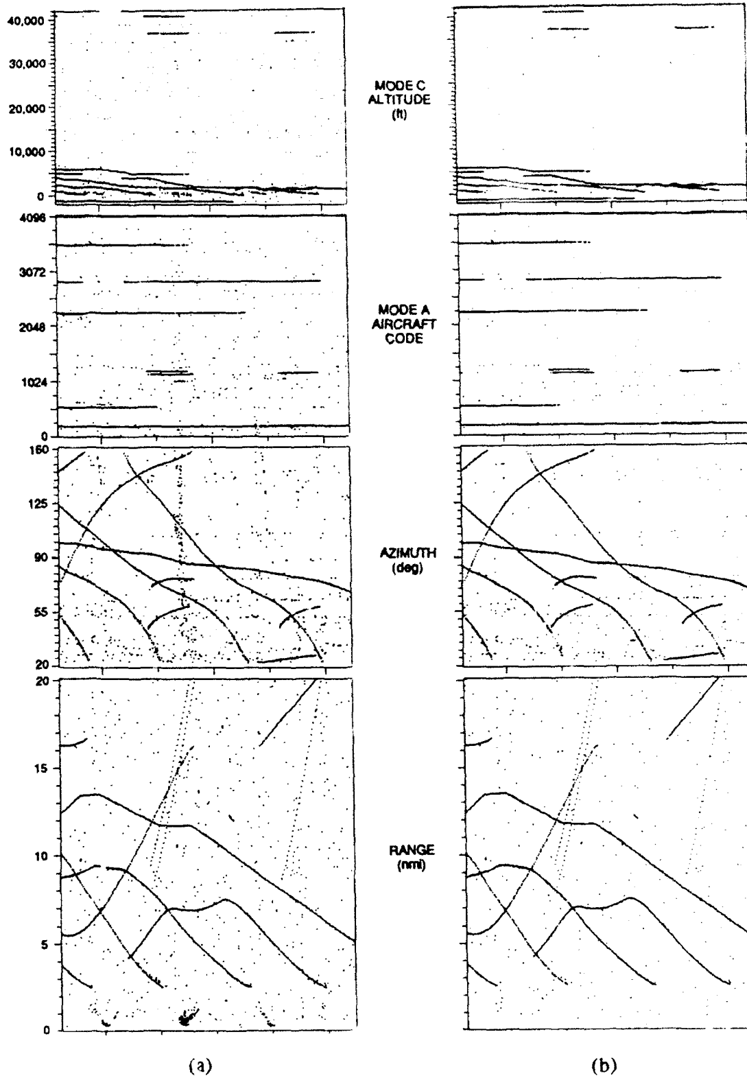
Figure 3. Representative reply information from the East quadrant. (a) all replies. (b) ungarbled replies.
