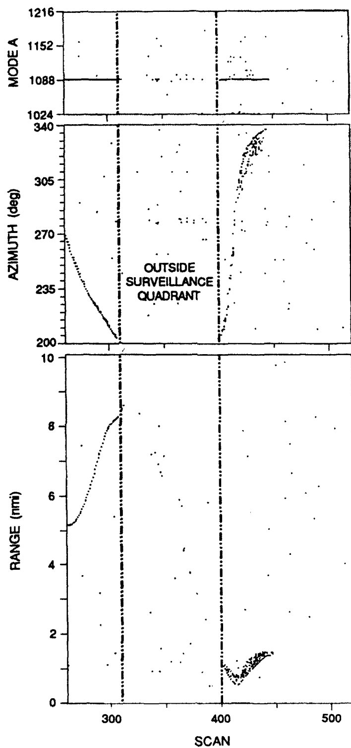
Figure 9. Valid reply sequence for the arrival aircraft A2 from Figure 7.
