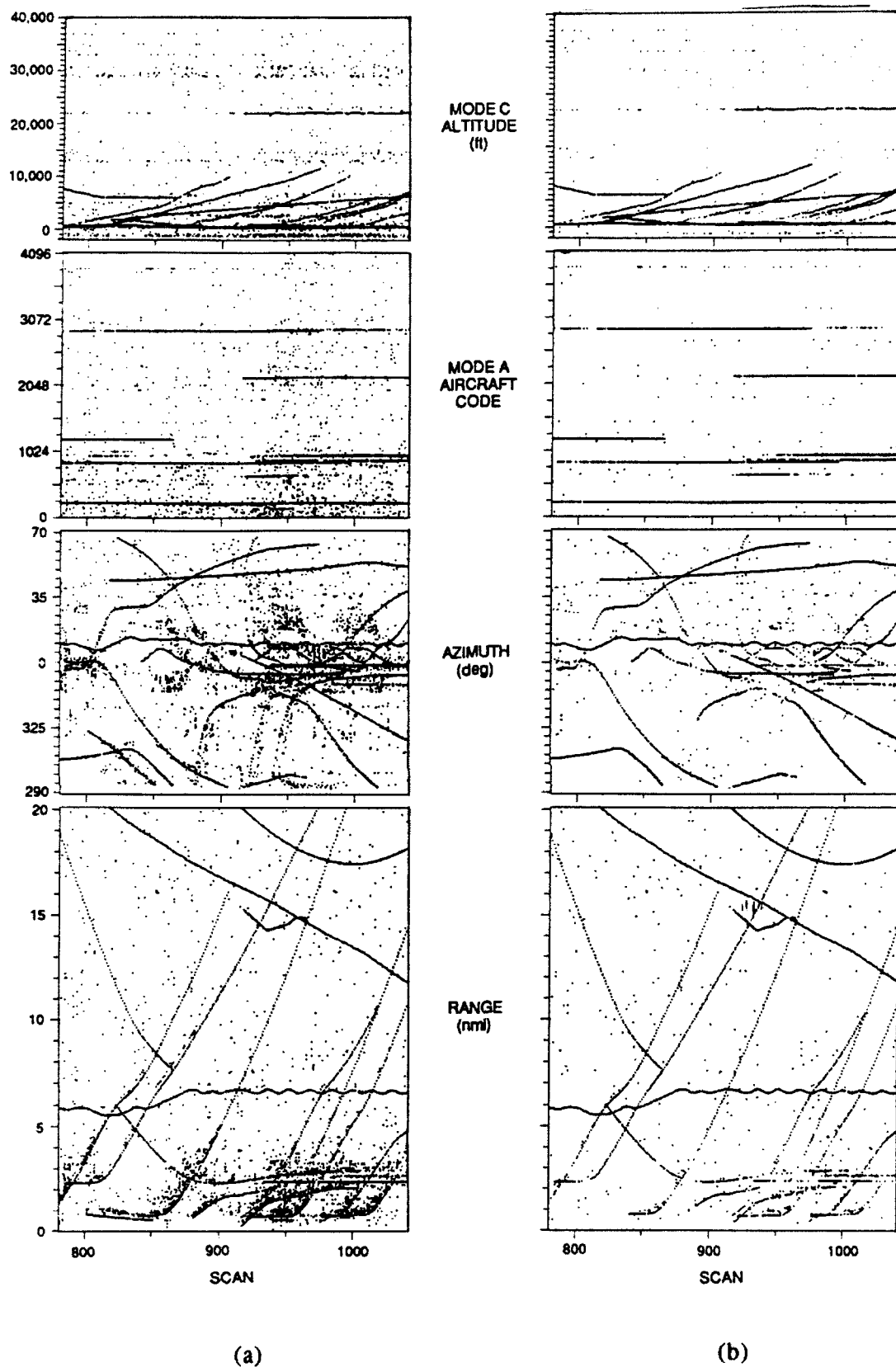
Figure 11. Representative reply information from the North quadrant. (a) all replies. (b) ungarbled replies.
