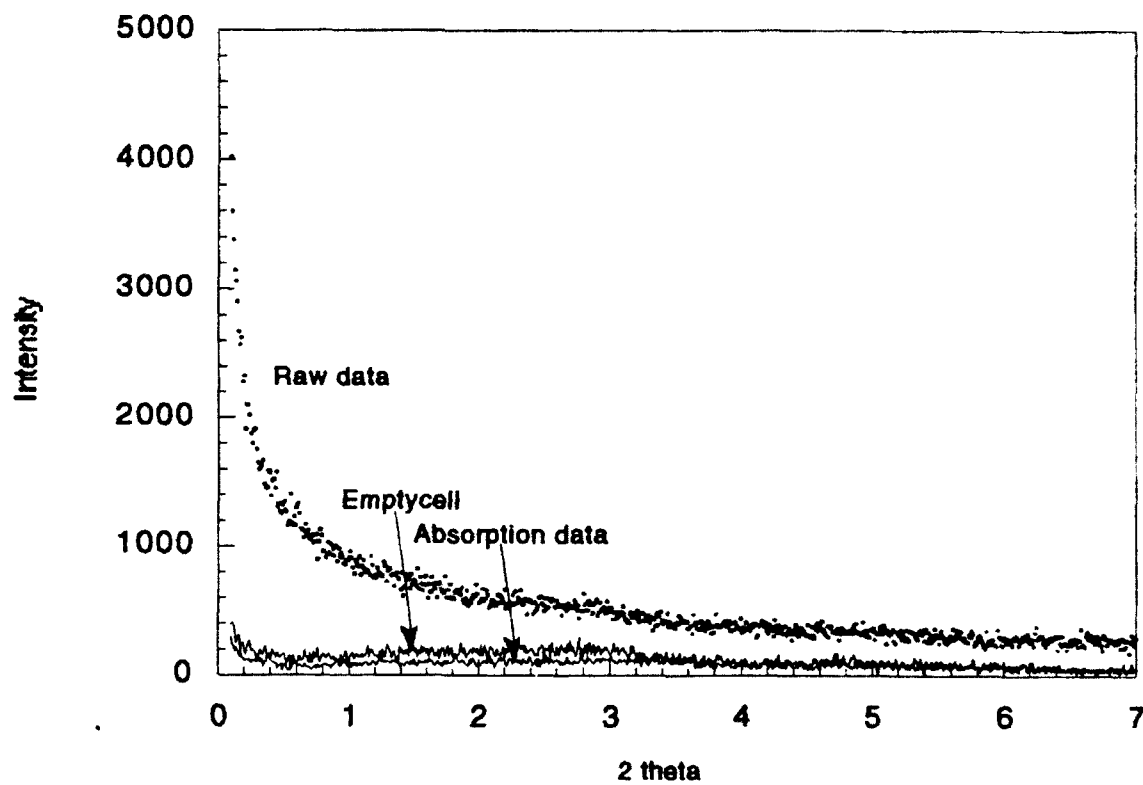
Figure 22. SAXS curves of AAM raw data, empty cell scattering and absorption data.
