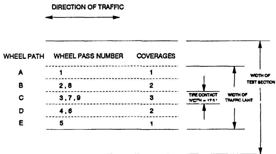
Figure 2. Traffic pattern for test Lanes 1 and 2
