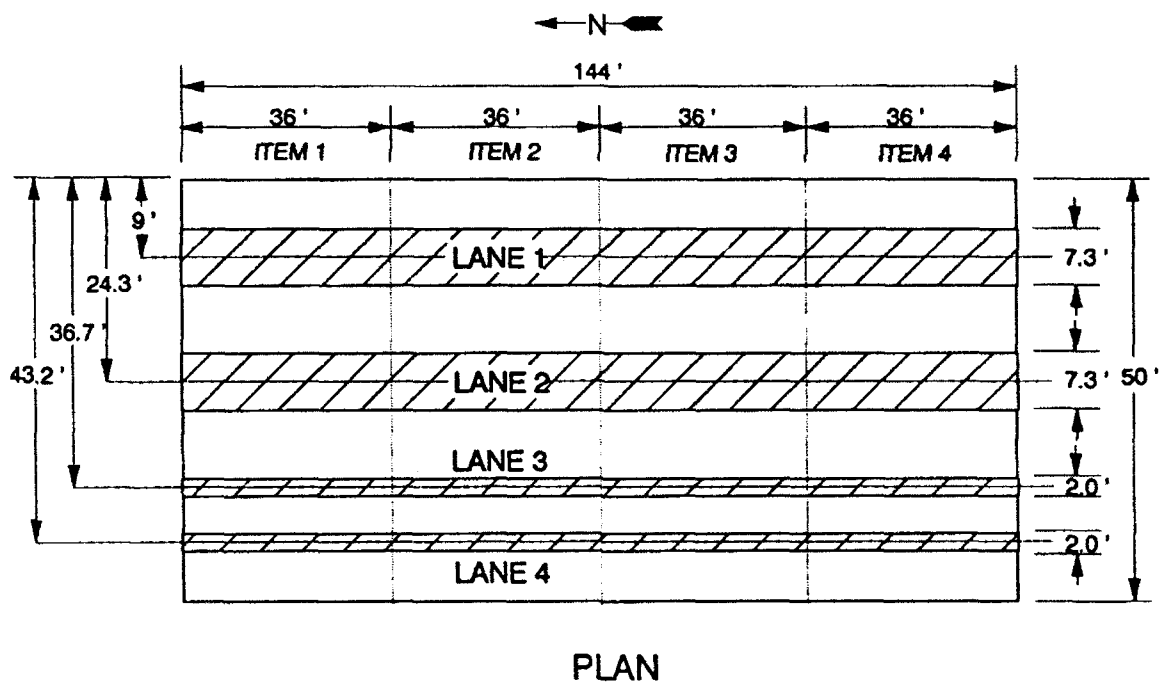
Figure 1. Layout of geogrid test section
