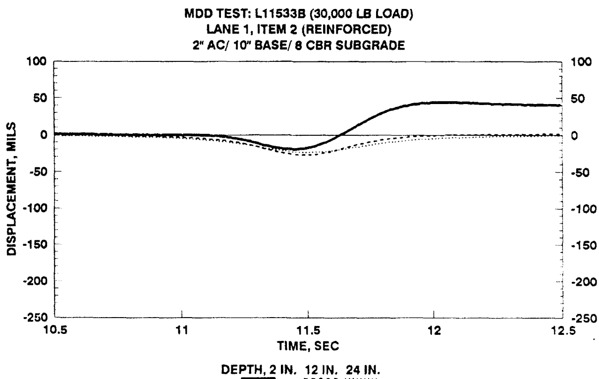
Figure 61. Displacements for pass 1533, wheel Path B
