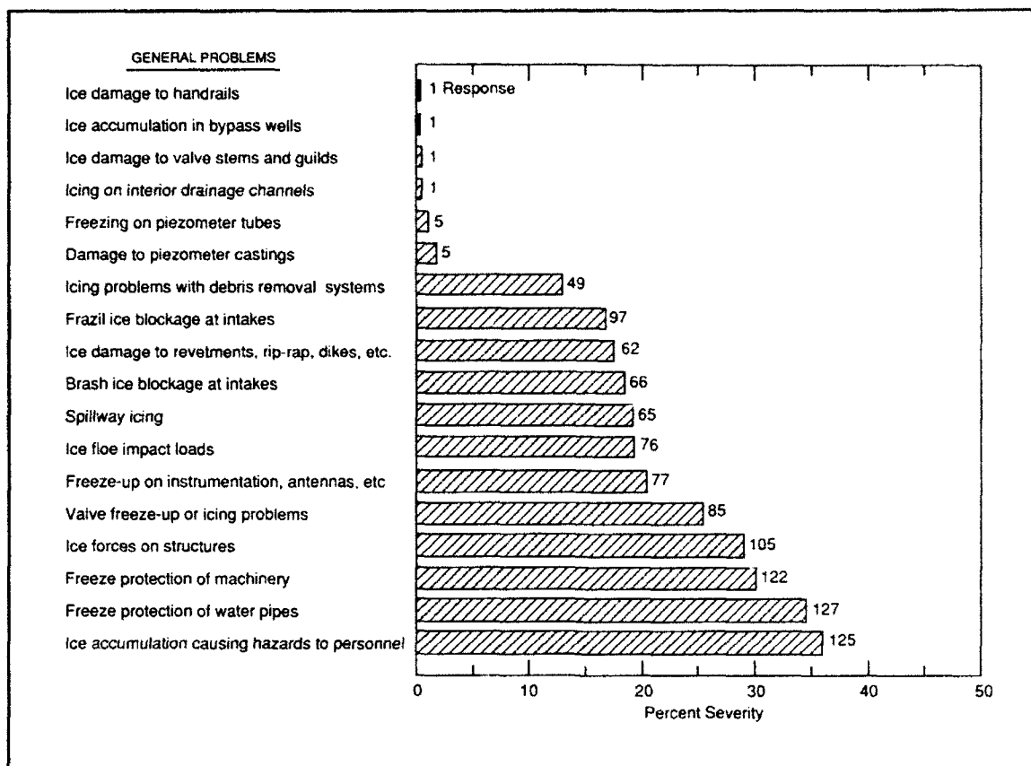
Figure 10. Severity of general ice problems
