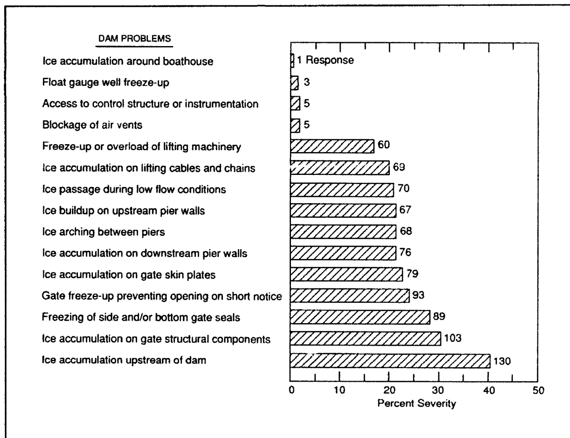
Figure 9. Severity of ice problems at dams
