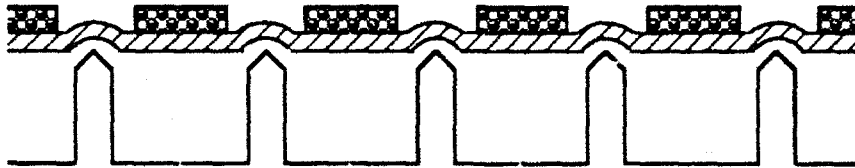
Step 7: Develop and strip photoresist
