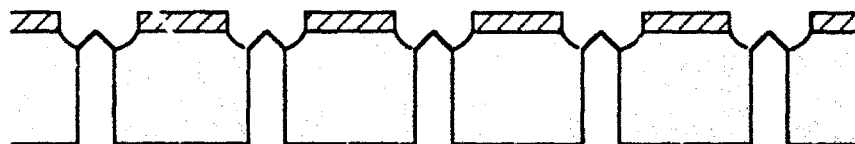
Step 10: Strip photoresist
