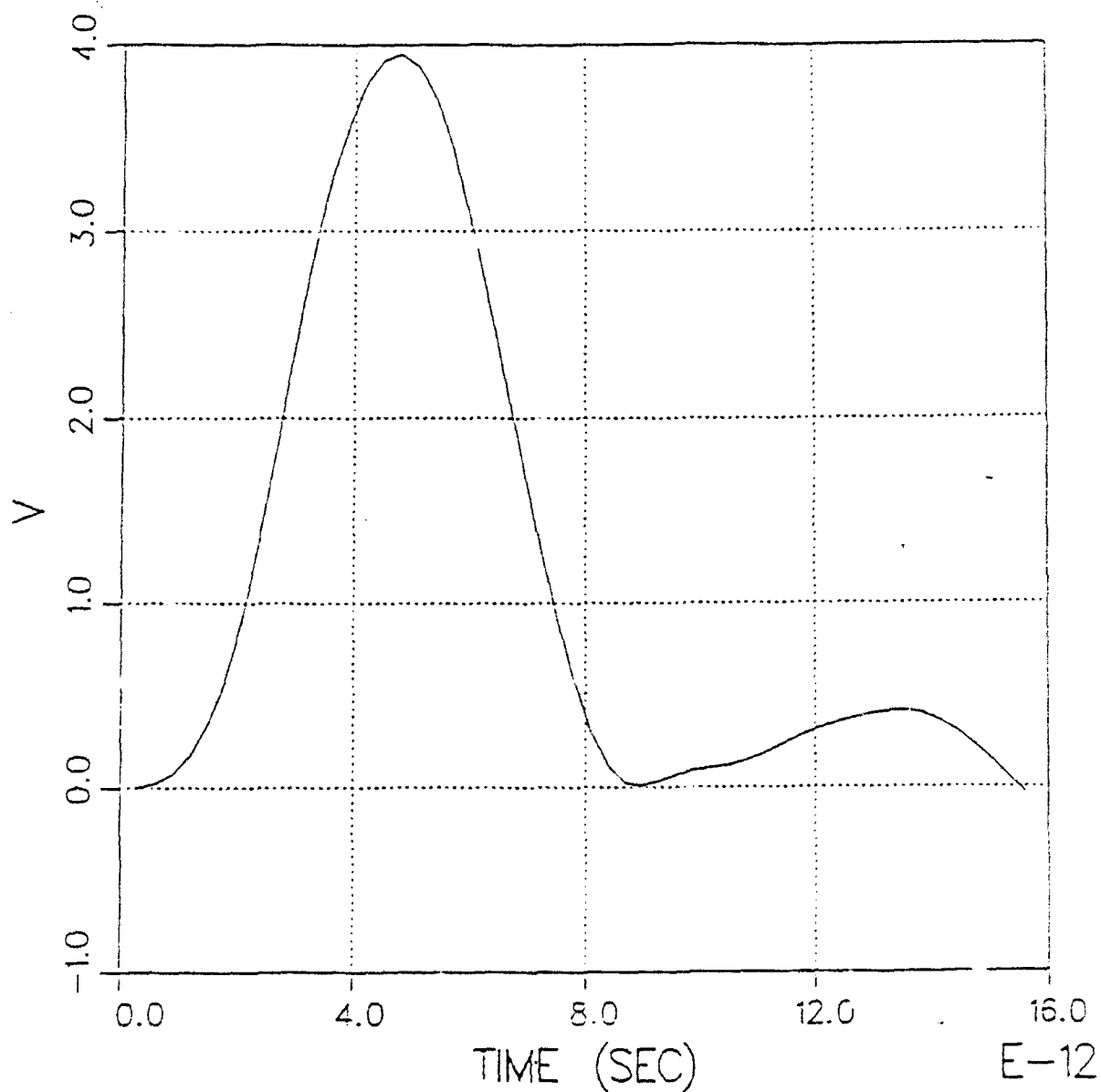
Figure 6.8. Incoming pulse.
