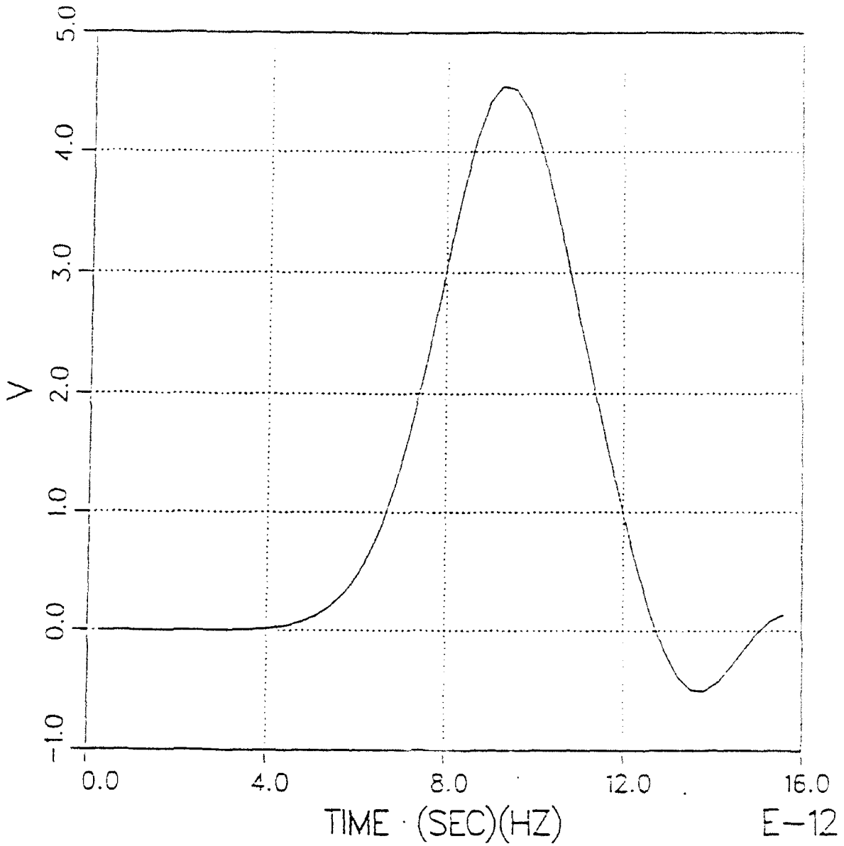
Figure 6.9. Transmitted pulse.
