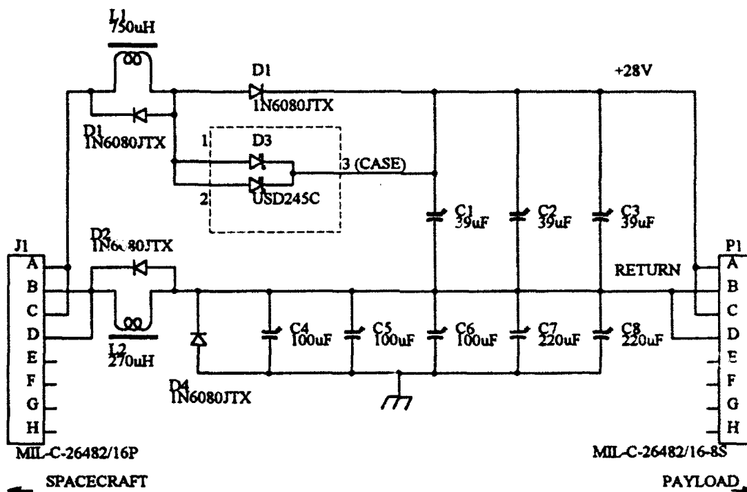
SPREE Power Filter - Final Version
