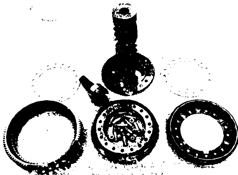
Figure 95. Components of Double Helical Pinion/Spur Gear Assembly
