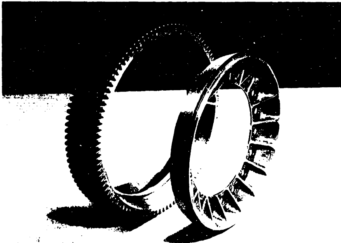
Figure 92. Spur Gear and Elastomeric Load Sharing Device
