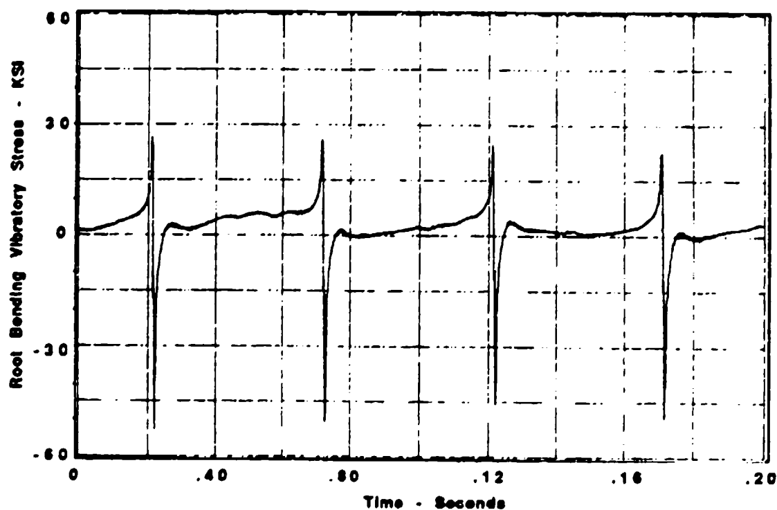
Figure 122. Stress vs Time, Upper Spur Gear, Gage #10
