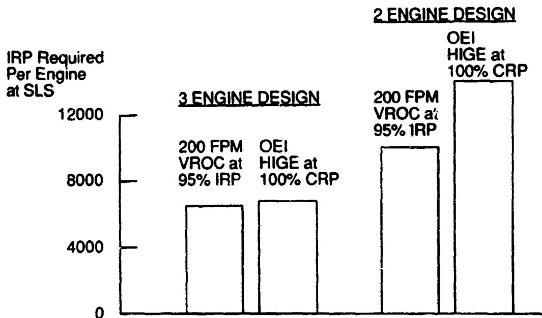
Figure 2. Power Required for Climb and OEI, 2 vs 3 Engines
