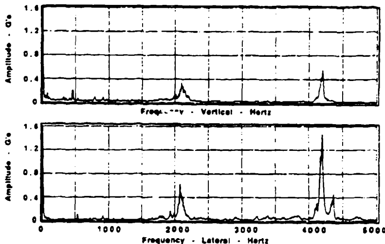
Figure 139. Typical Vibration Signatures, Steel Survey
