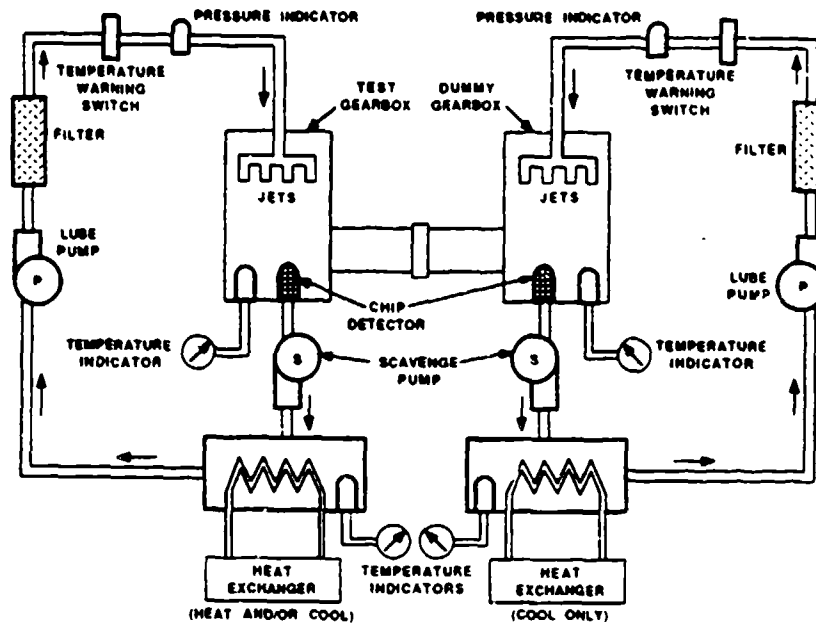
Figure 79. 1/2 Size Gearbox Lubrication System Schematic
