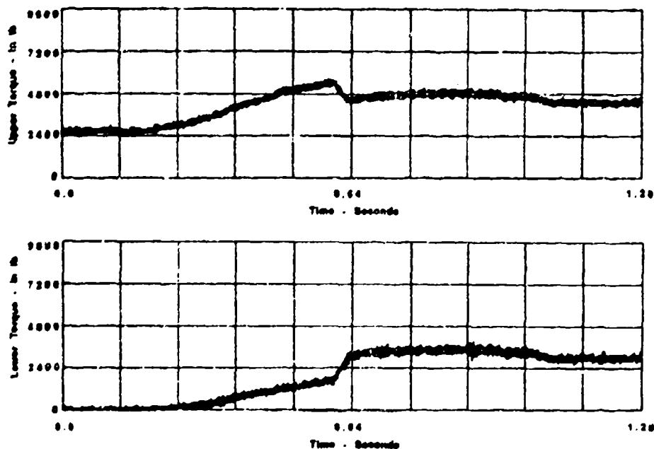
Figure 138. Idler Shaft Torque vs Time, Steel Survey
