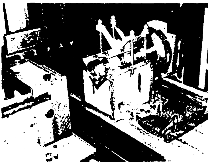
Figure 93. Double Helical Pinion in Horizontal Boring Machine
