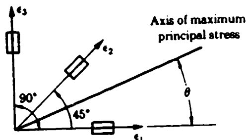
Figure 173. Rectangular Strain Gage Rosette
