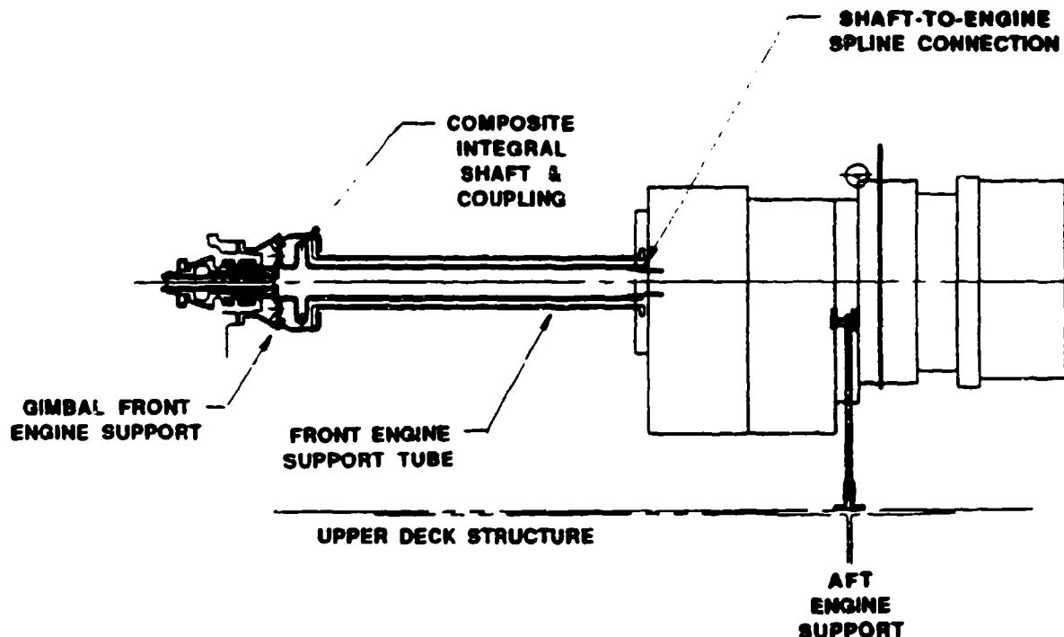
Figure 44. ART/ACA Engine Installation
