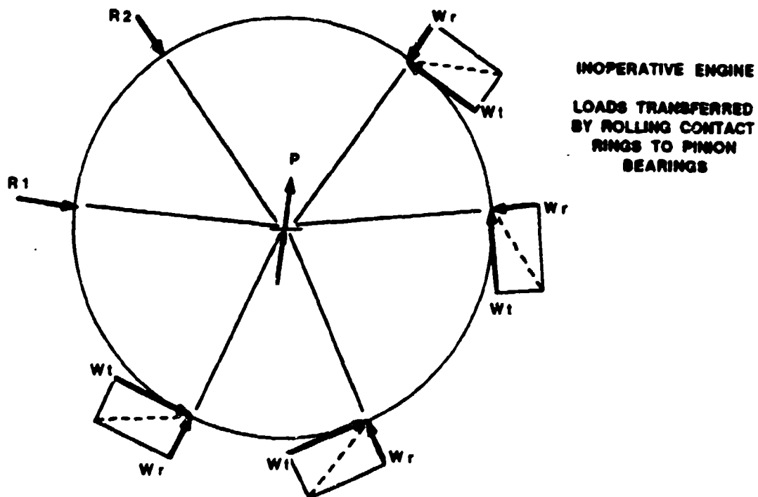
Figure 29. Bull Gear Reaction, One Engine Inoperative
