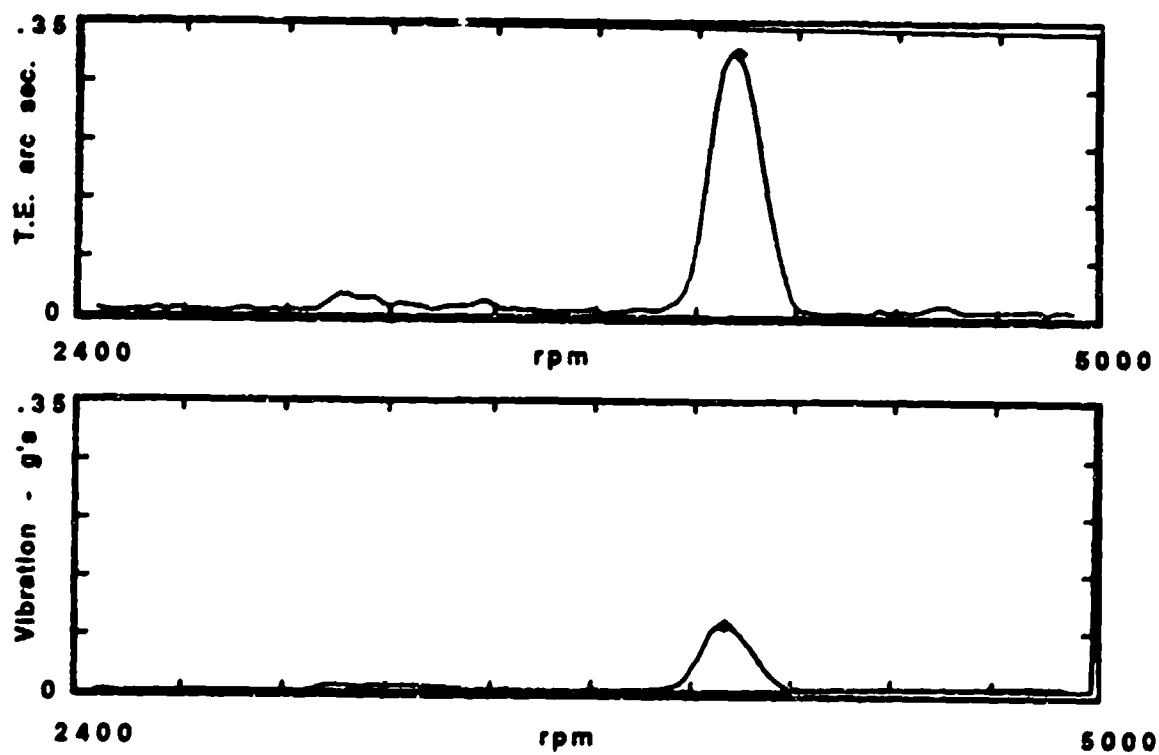
Figure 145. Lower D Hel TE vs Upper Lat Vib, Steel @ 100% Torque
