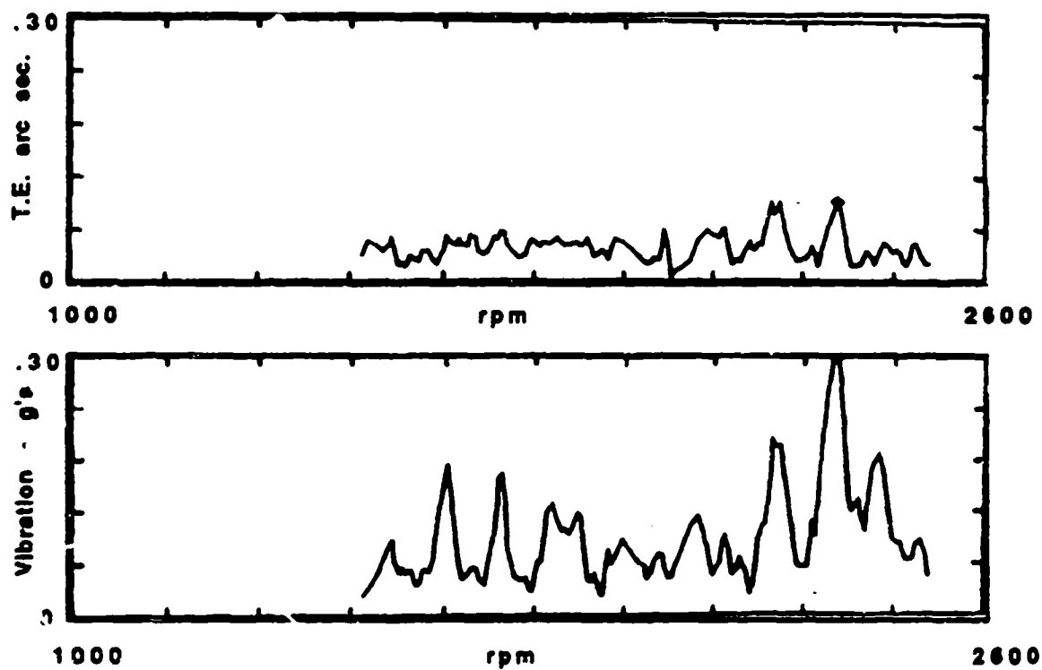
Figure 144. Lower Spur TE vs Upper Lat Vib, Steel @ 100% Torque
