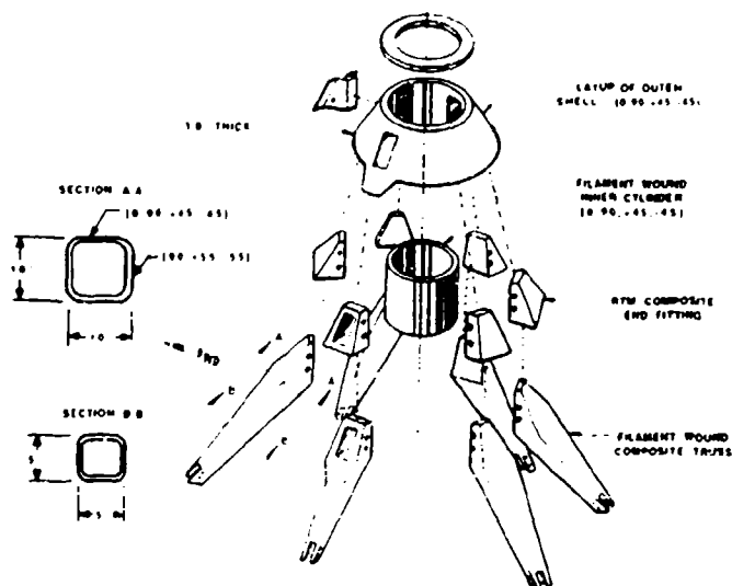
Figure 38. Schematic of Standpipe Structure Separate Parts
