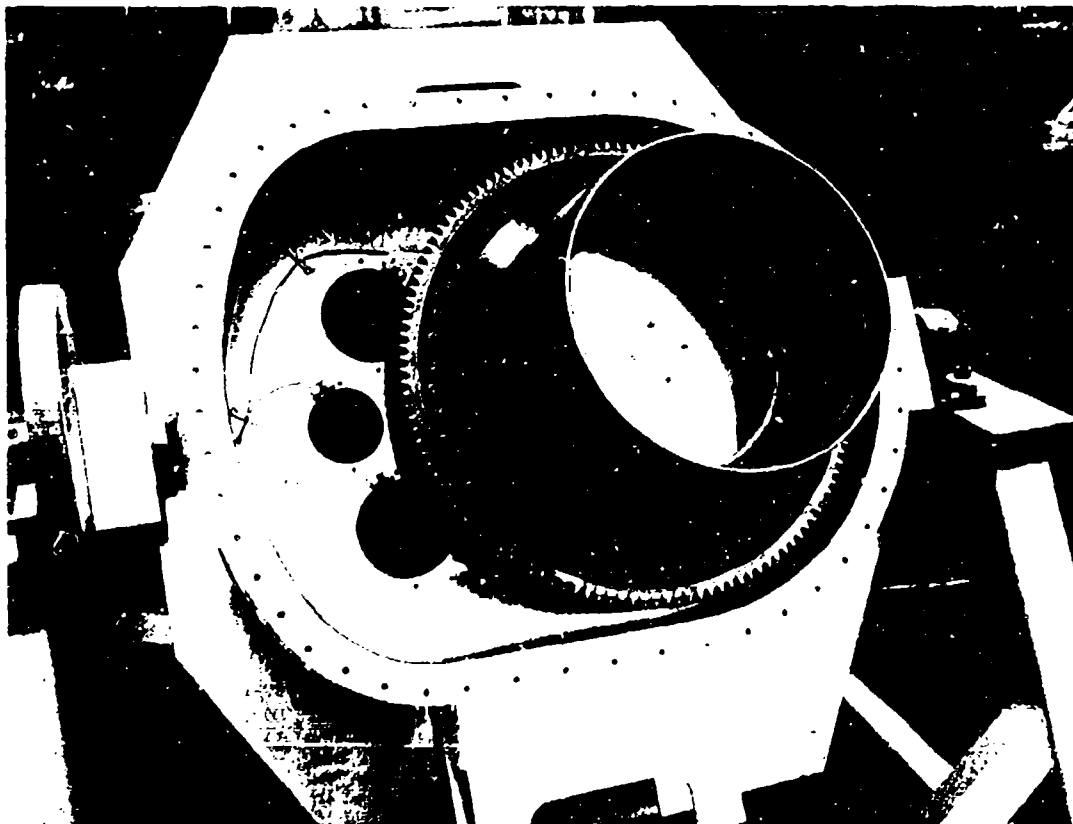
Figure 99. 1/2 Output Double Helical Bull Gear in Housing
