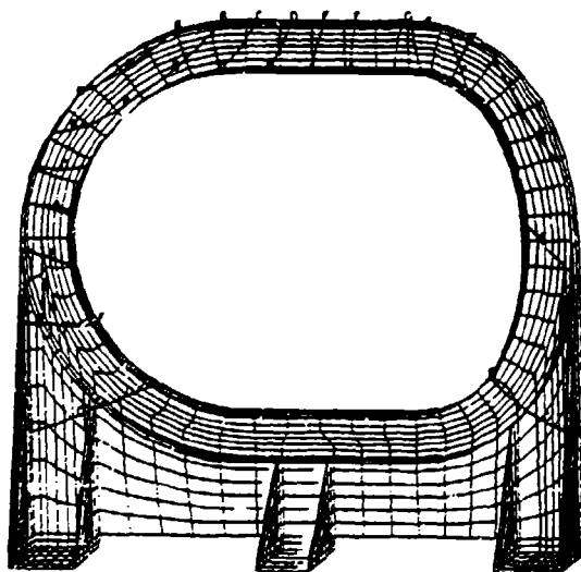
Figure 67. Test Fixture Total Deflection
