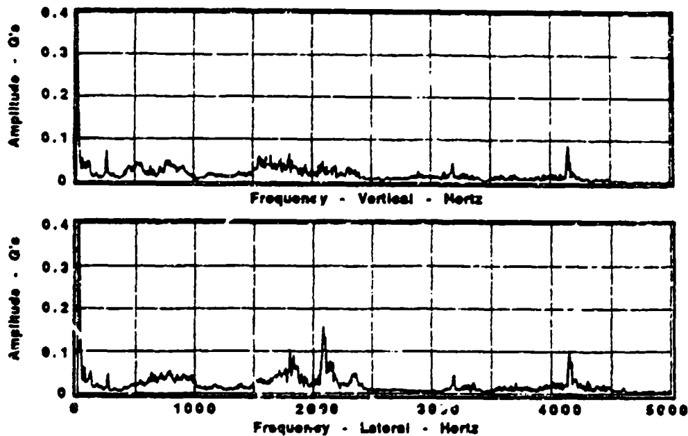
Figure 117. Typical Vibration Signature, No Load
