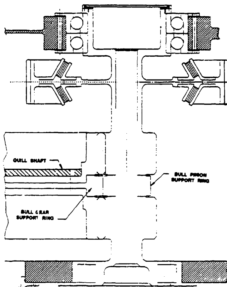
Figure 32. Bearingless Bull Gear Design
