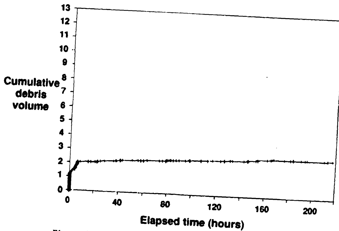
Figure 176. Long Term Trend of Particles Accumulated
