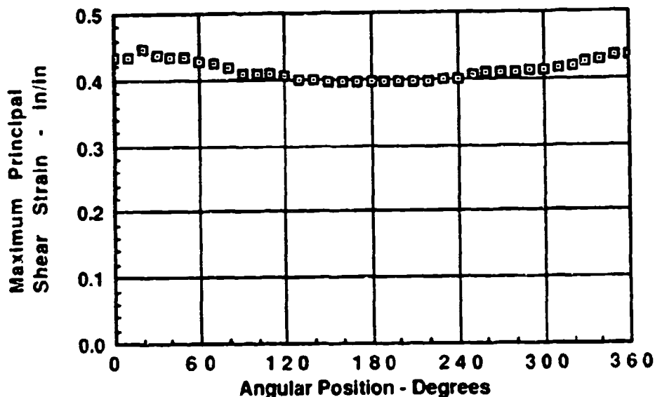
Figure 77. Maximum Principal Shear Strain vs Angular Position
