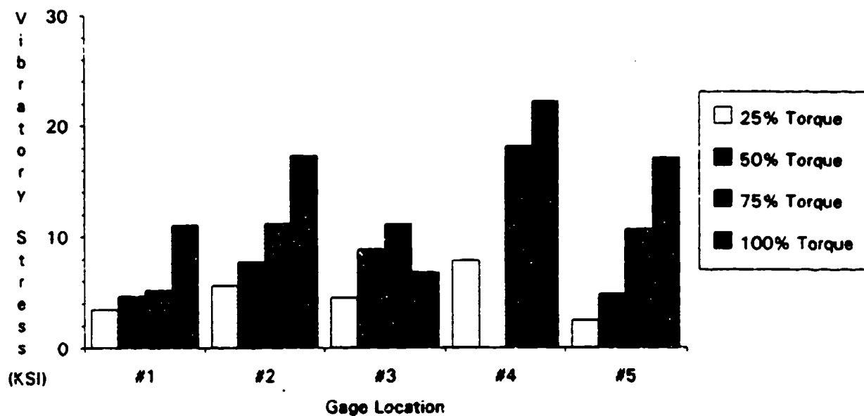
Figure 127. Vibratory Stress, Spur Pinion Meshing w/Upper Spur Gear
