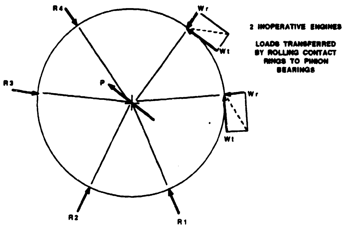
Figure 30. Bull Gear Reaction, Two Engines Inoperative
