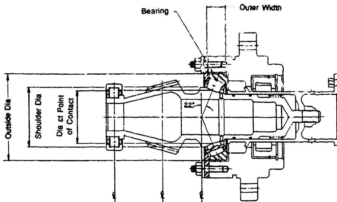
Figure 36. Mounting of Angular Contact Spherical Roller Bearing
