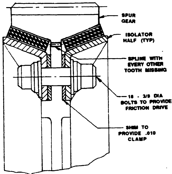
Figure 19. Inverted Elastomeric Torsional Load Sharing Device
