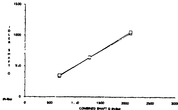
Figure 118. Load Sharing, Initial Pattern Development Survey
