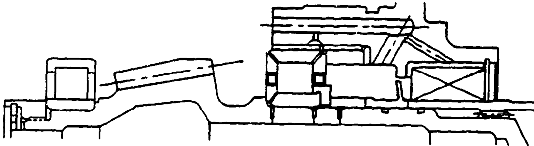
CYLINDRICAL ROLLER BEARING WITH THRUST CAPABILITY
