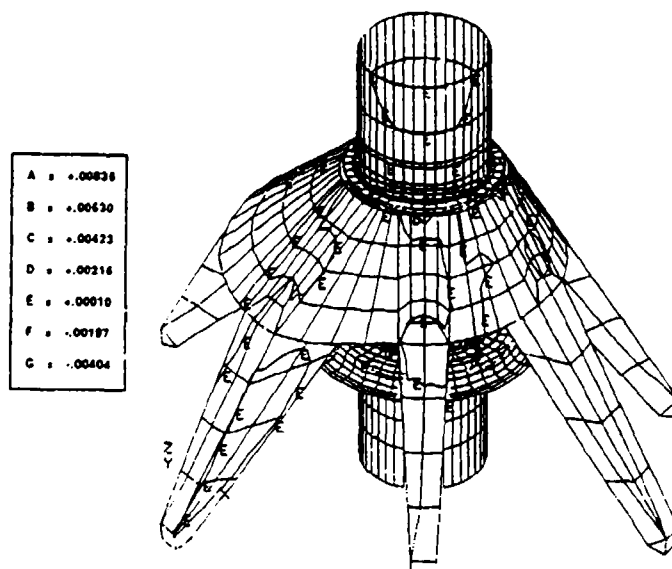
Figure 57. Composite Standpipe/Truss Strain in the Y Direction
