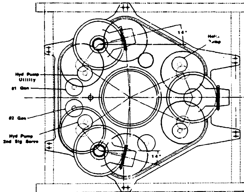
Figur 49. ART Main Gearbox Top View
