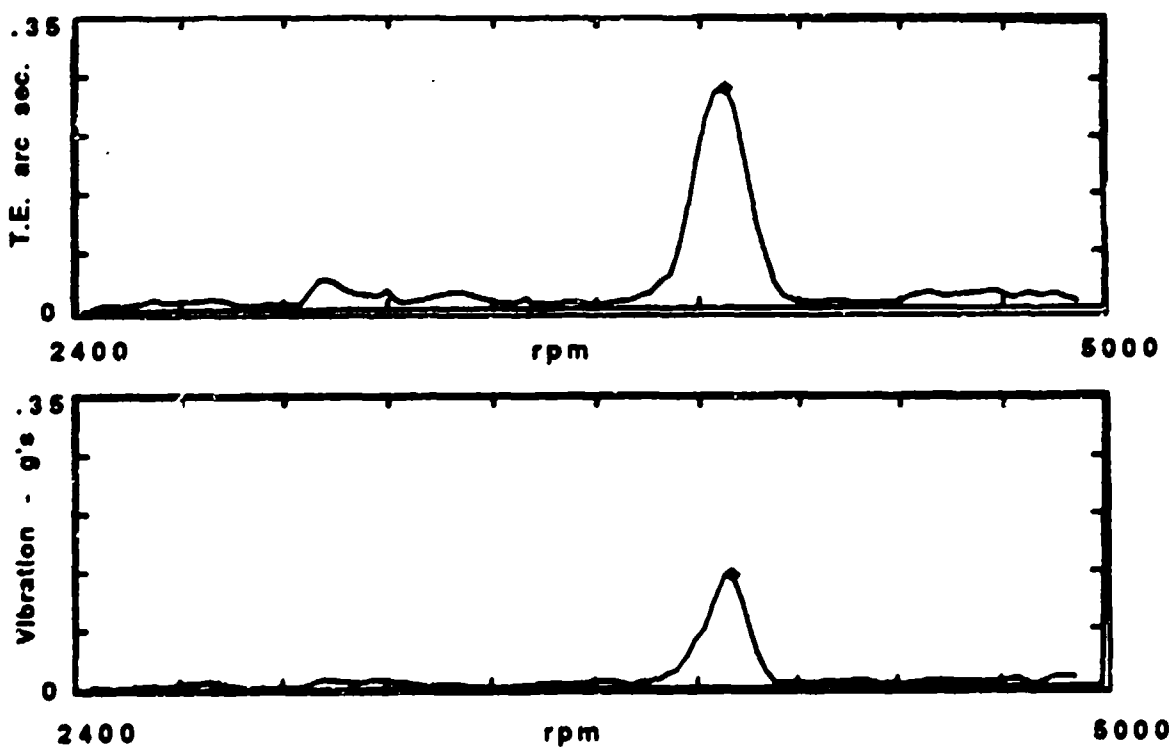
Figure 143. Lower D Hel TE vs Upper Lat Vib, Elastomer @ 100% Torque
