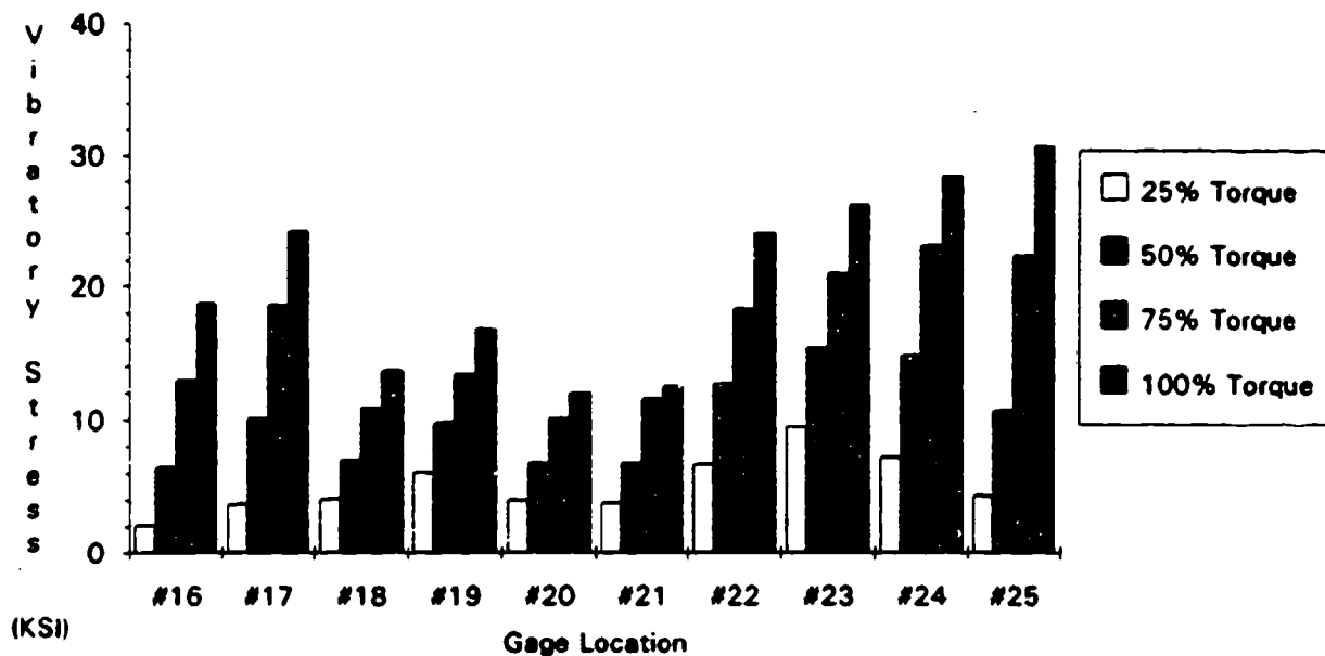
Figure 131. Vibratory Stress, Upper Double Helical Pinion
