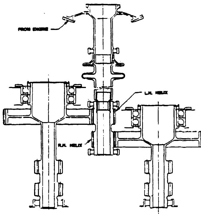
Figure 16. Helical Gear Load Sharing Scheme
