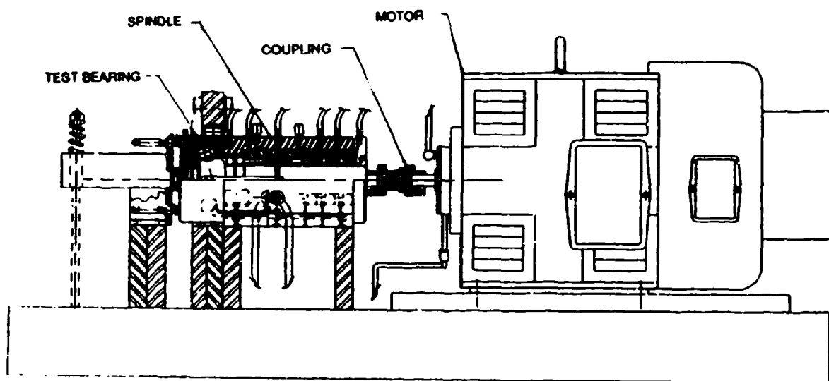
Figure 113. Schematic of Bearing Test Facility
