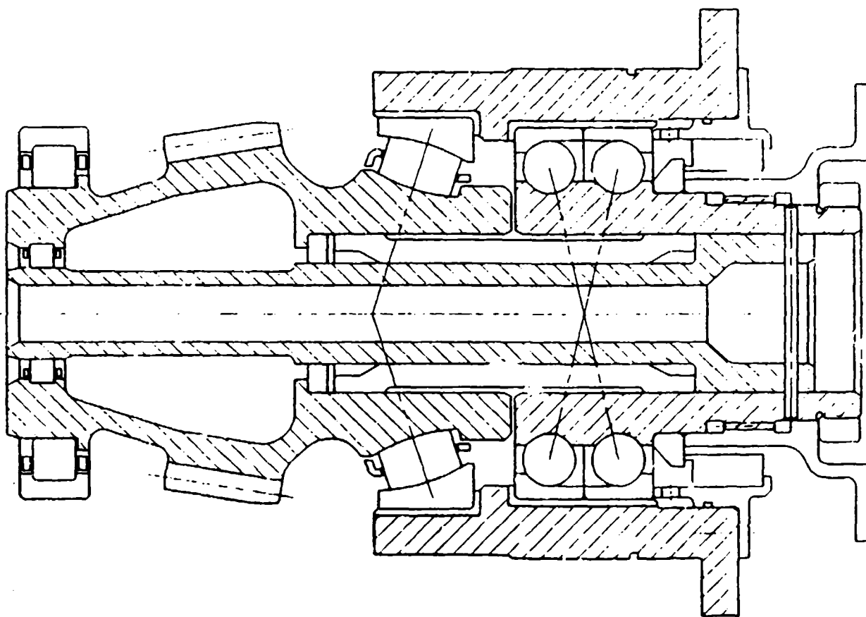
Figure 23. ART Input Bevel Pinion With Spring Clutch
