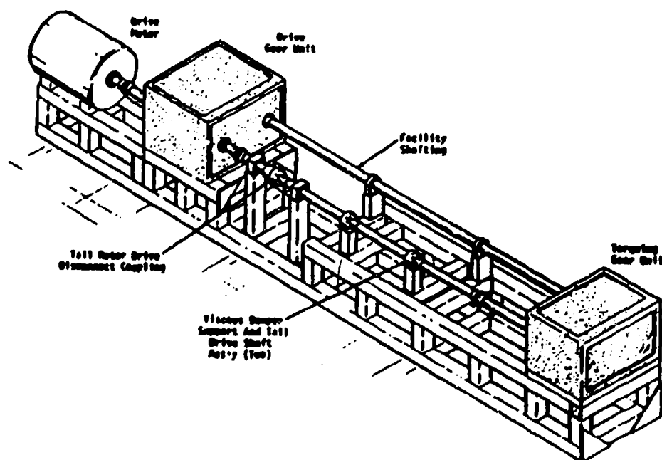
Figure 105. Shaft/Coupling Test Facility
