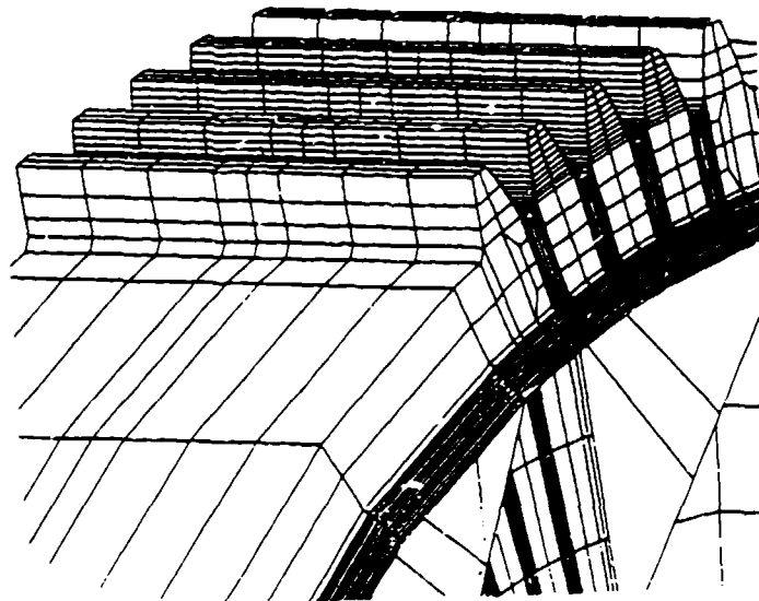
Figure 81. FEA Model of Input Spur Gear
