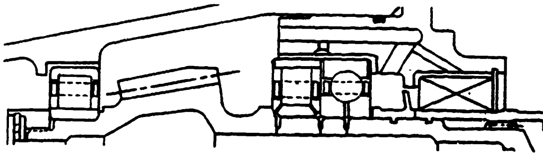
BALL/ ROLLER BEARING COMBINATION
