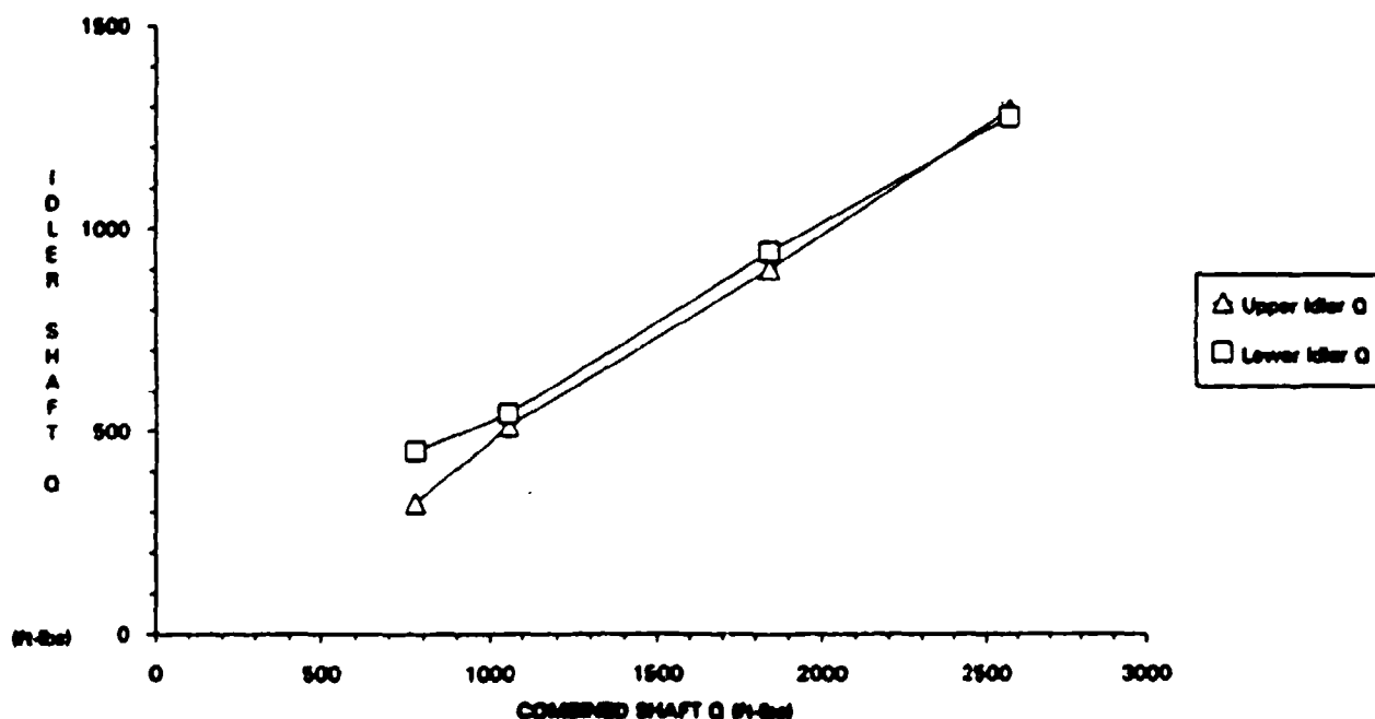
Figure 120. Load Sharing, Final Pattern Development Survey
