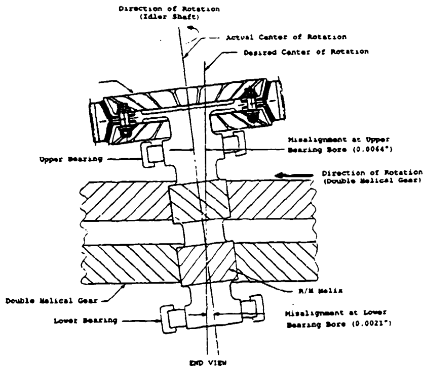
Figure 162. Illustration of Shaft Misalignment
