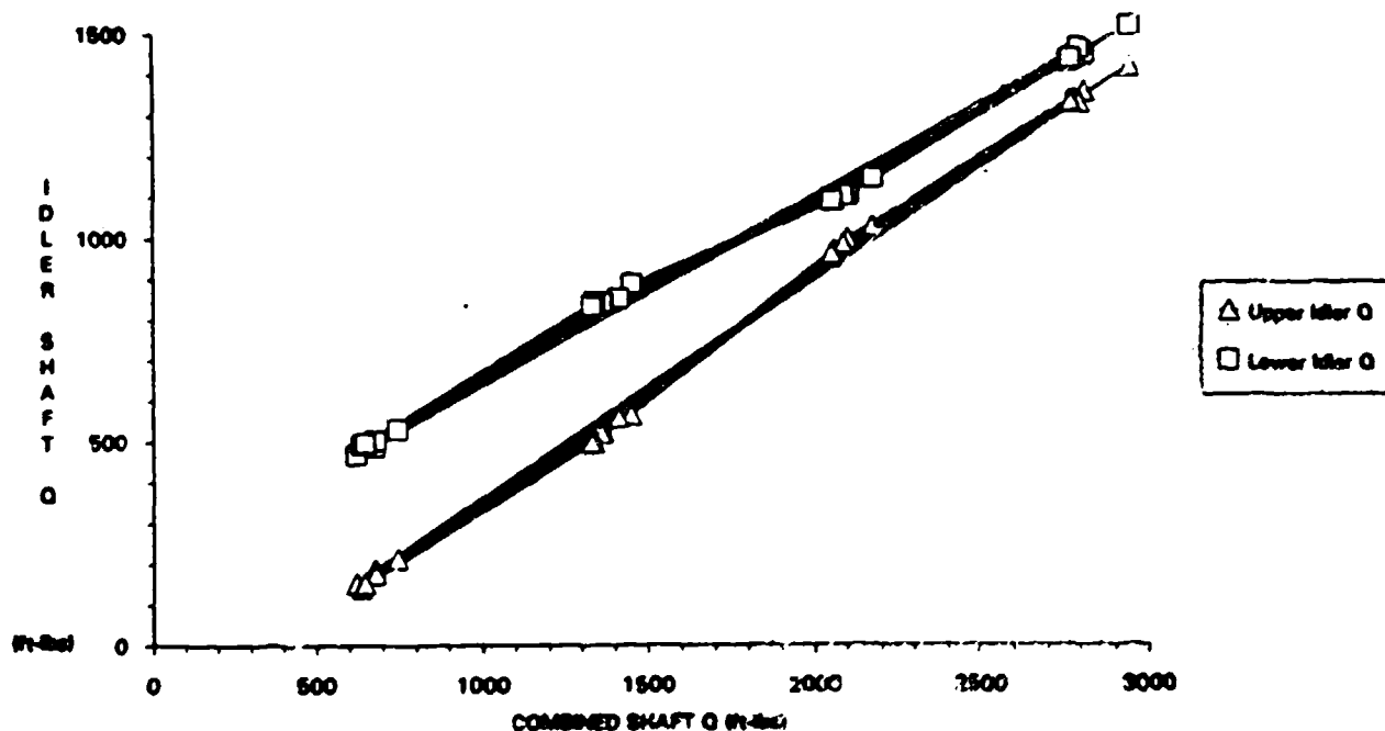
Figure 136. Load Sharing, 2nd Half of Dynamic Surveys
