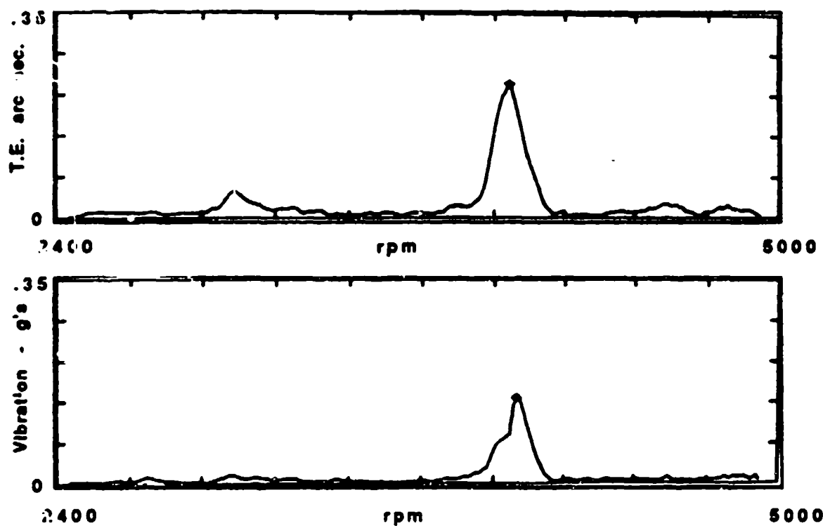
Figure 142. Upper D Hel TE vs Upper Lat Vib, Elastomer @ 100% Torque
