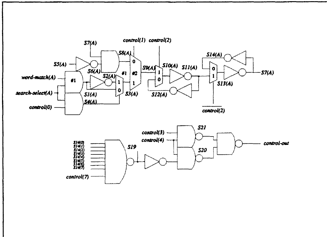
Figure 18. Match-Circuit Schematic.
