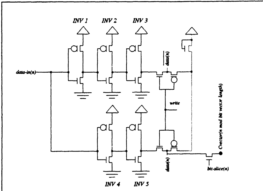
Figure 22. Bit-Serial Word-Parallel Associative-Memory Architecture Write-Circuit Schematic.
