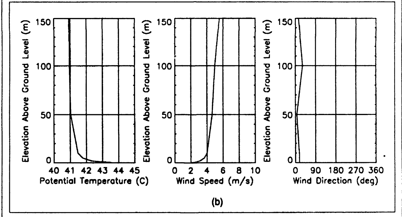
Figure A5. WSMR stable (a) and unstable (b) meteorological upper air initialization data correlated with the surface observation data in Tables A5.1 and A5.2, respectively.
