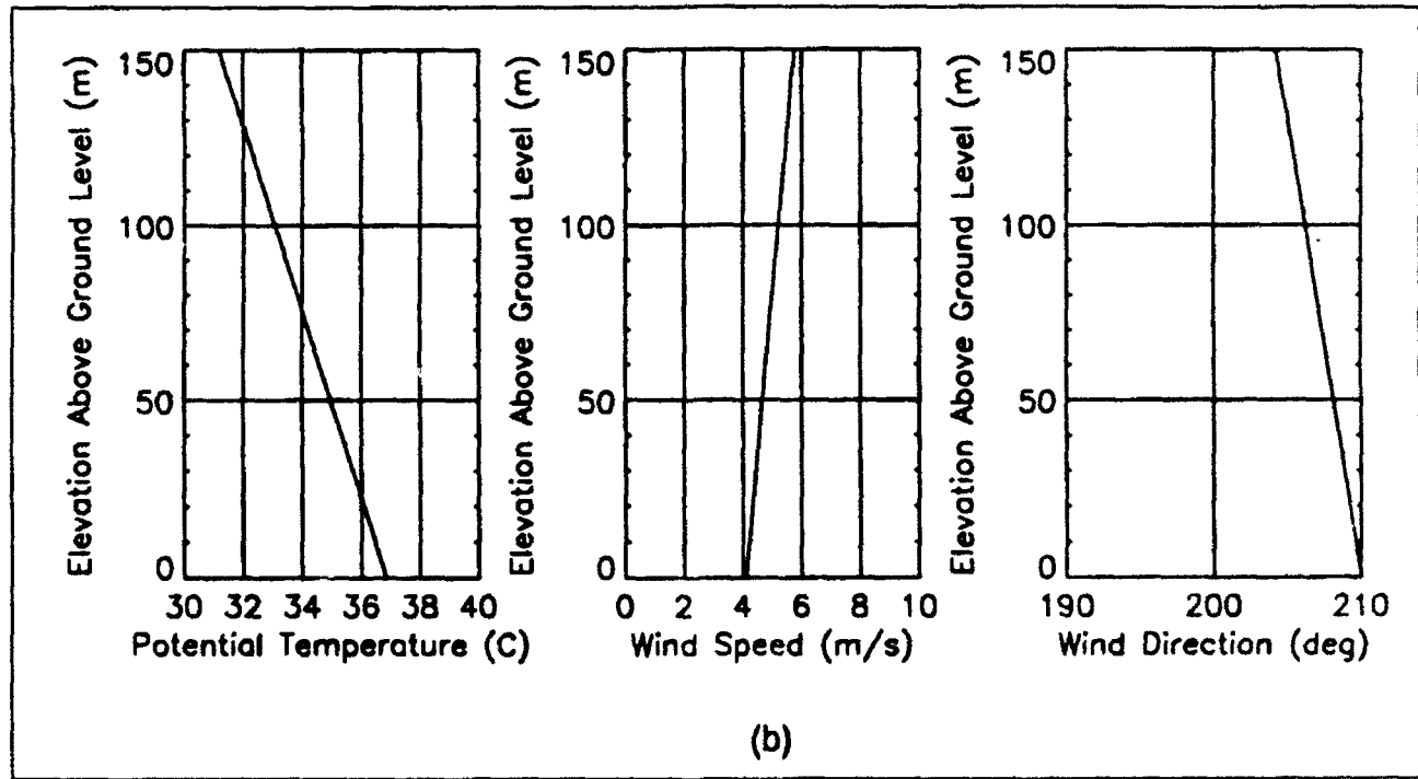
Figure A7. Project WIND stable (a) and unstable (b) meteorological upper air initialization data correlated with the surface observation data in Tables A7.1 and A7.2, respectively.
