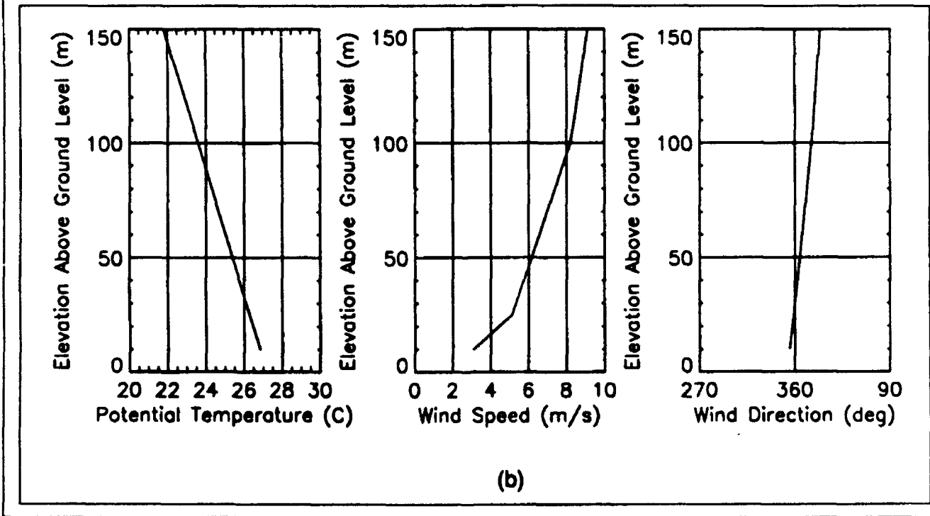
Figure A6. NTC stable (a) and unstable (b) modeled upper air initialization scheme that was correlated with the surface observation data in Tables A6.1 and A6.2, respectively, for observation site S-1 (Fig. A2 and Table A2).
