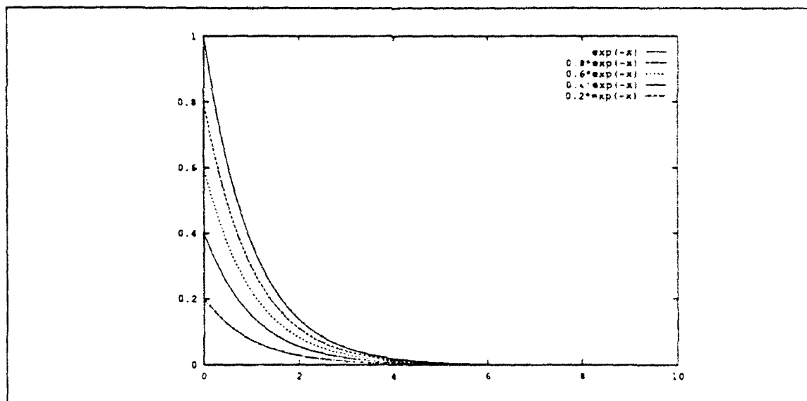
Figure 2. Single term exponential with varying A.
