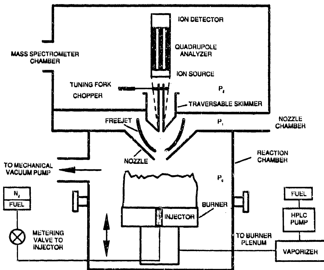
Fig. 1 Molecular Beam Apparatus
